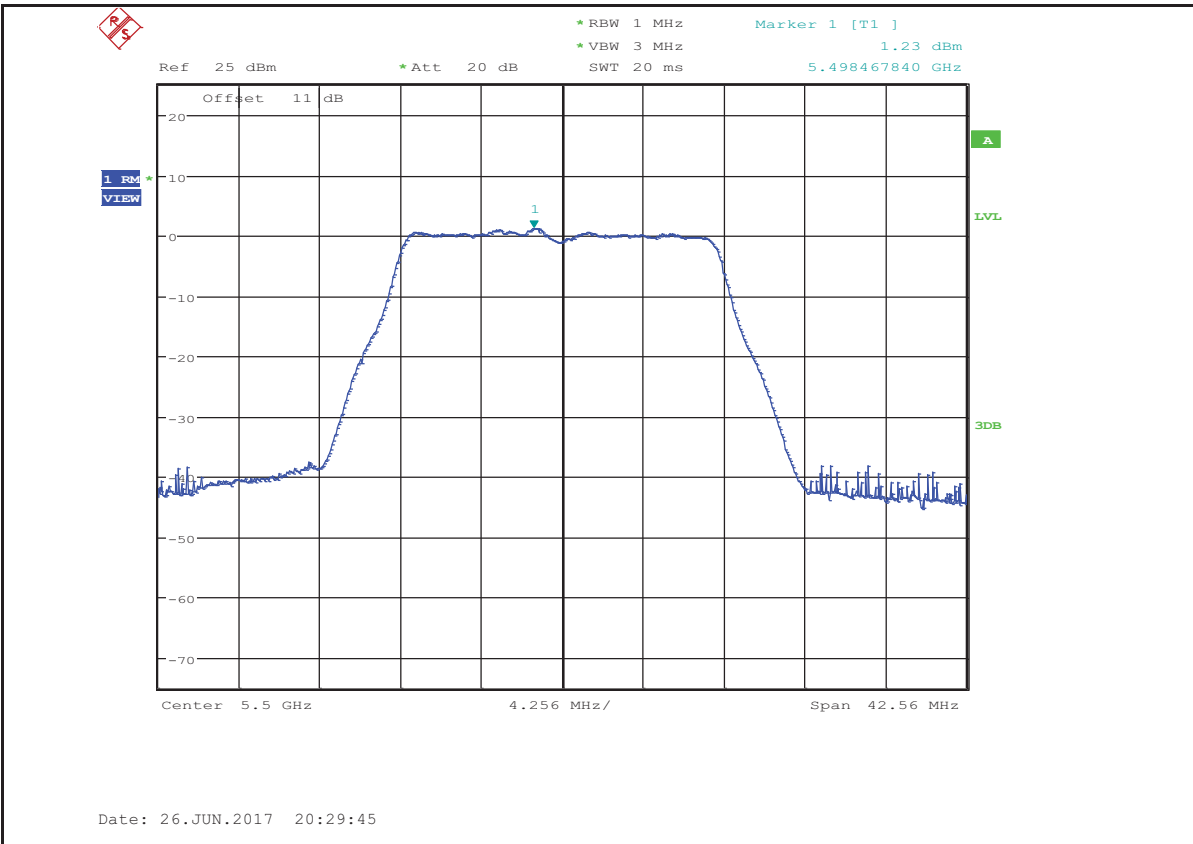
Maximum Power Spectral Density_TNVN_11AMIMO_5500_Ant1+Ant2
