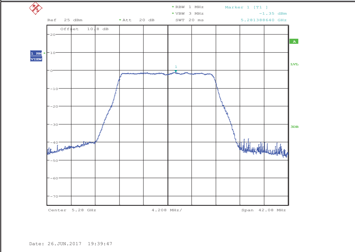
Maximum Power Spectral Density_TNVN_11AMIMO_5280_Ant2
