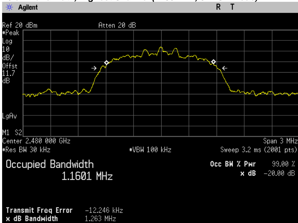
20 dB Bandwidth, Highest Channel (2480 MHz, 8DPSK Mode)
