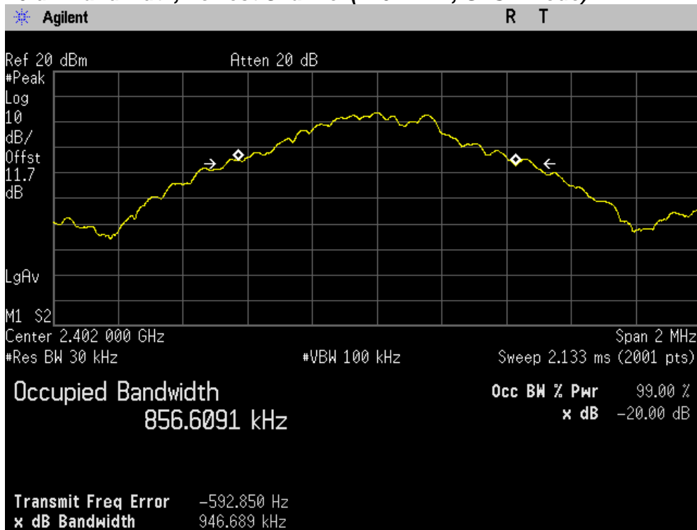
20 dB Bandwidth, Lowest Channel (2402 MHz, GFSK Mode)
