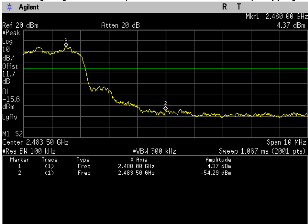
Band Edge Highest Channel(2480 MHz, \pi/4 DQPSK Mode)_Hopping mode
