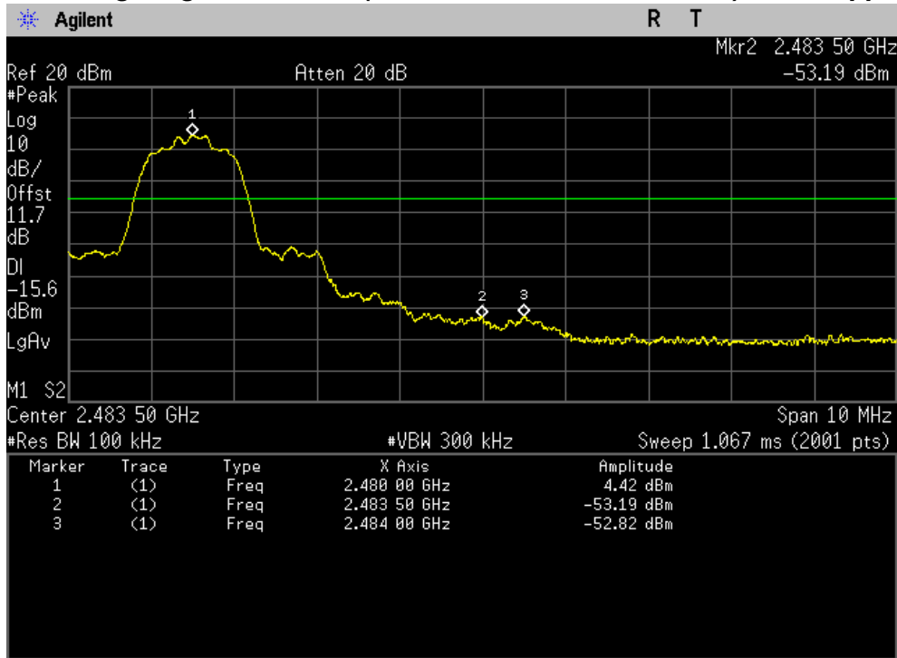
Band Edge Highest Channel(2480 MHz, \pi/4 DQPSK Mode)_Non-hopping mode
