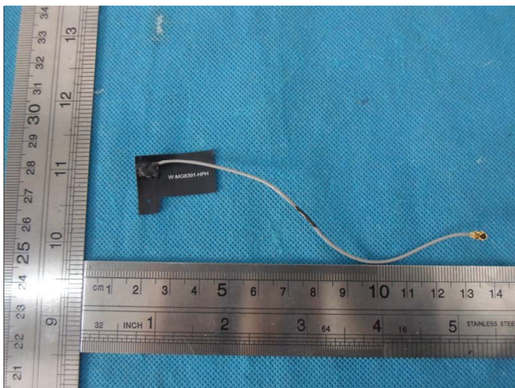
Photo 12 BT Antenna
