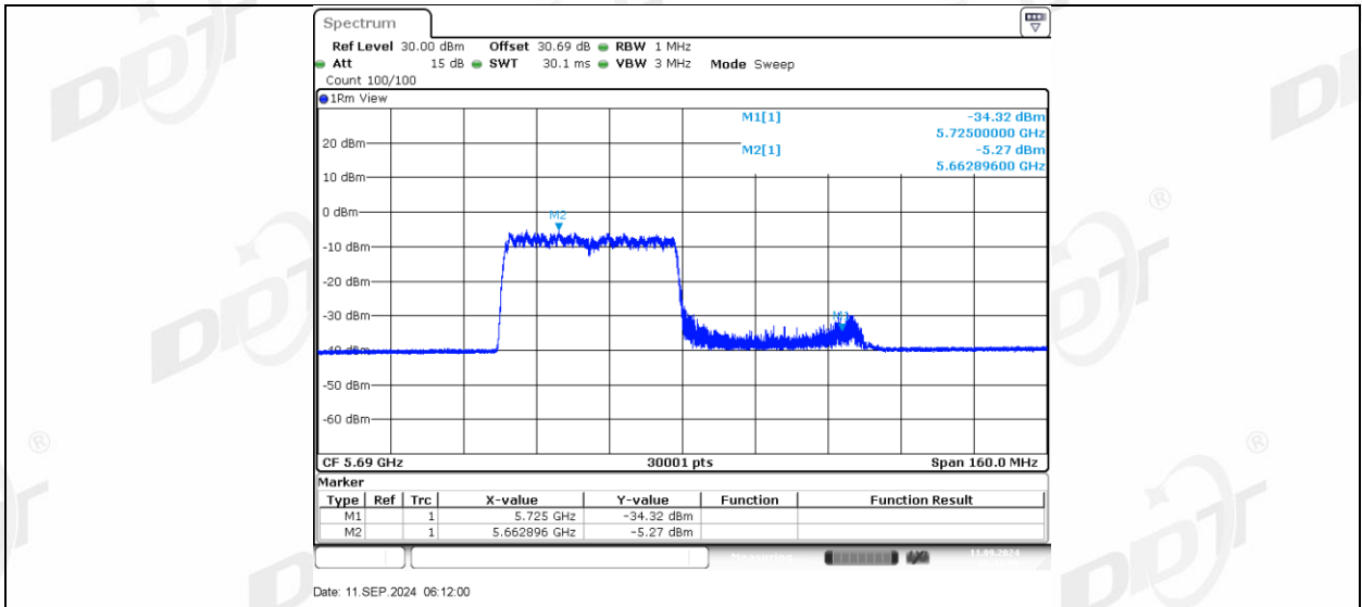
11AX80MIMO Ant1_5690_UNII-2C_484Tone_RU66
