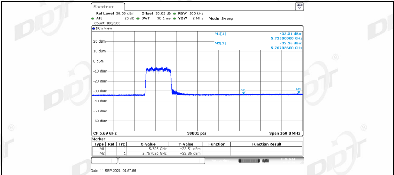
11AX80MIMO Ant1 5690 UNII-3 242Tone RU64
