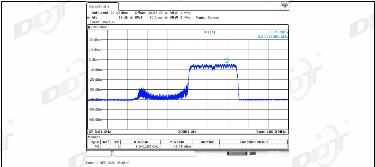
11AX80MIMO Ant1_5690_UNII-2C_242Tone_RU61
