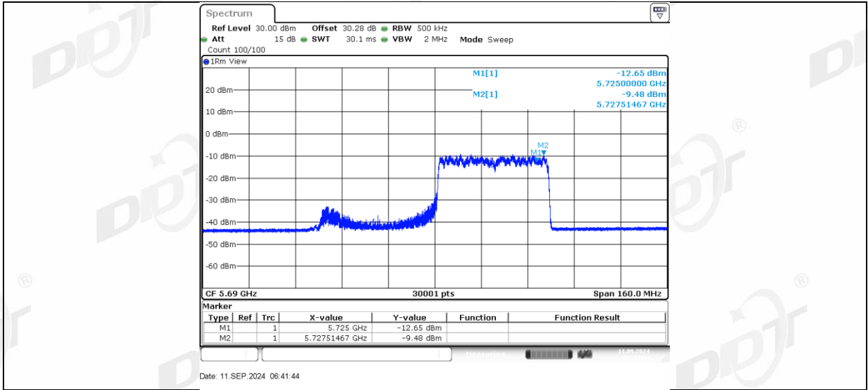
11AX80MIMO Ant2 5690 UNII-3 242Tone RU61
