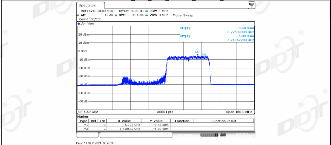
11AX80MIMO Ant1 5690 UNII-3 242Tone RU61
