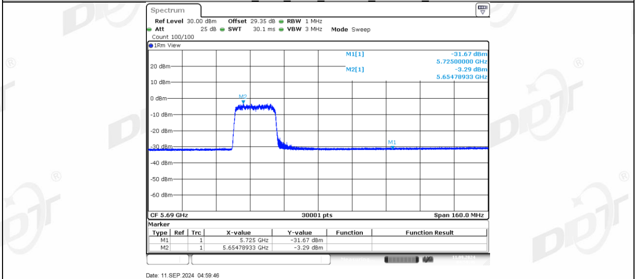
11AX80MIMO Ant2_5690_UNII-2C_242Tone_RU64
