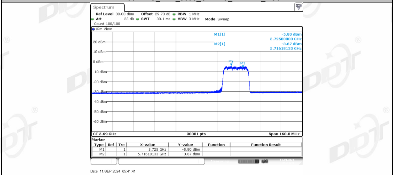
11AX80MIMO Ant1_5690_UNII-2C_484Tone_RU65
