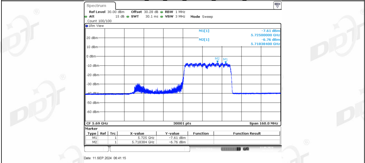
11AX80MIMO Ant2_5690_UNII-2C_242Tone_RU61
