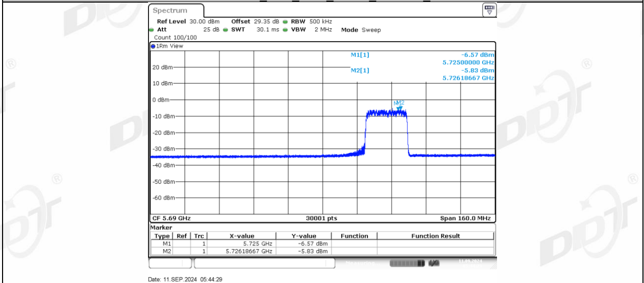
11AX80MIMO Ant2 5690 UNII-3 484Tone RU65
