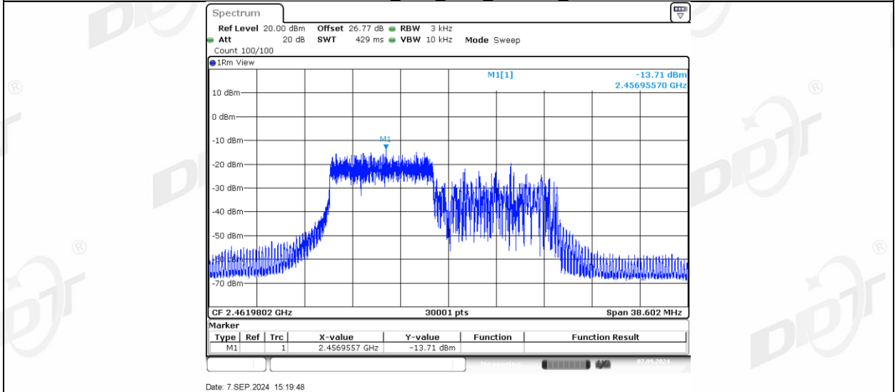
11AX20MIMO Ant1 2462_106Tone RU54
