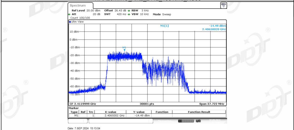
11AX20MIMO Ant2 2412_106Tone RU54
