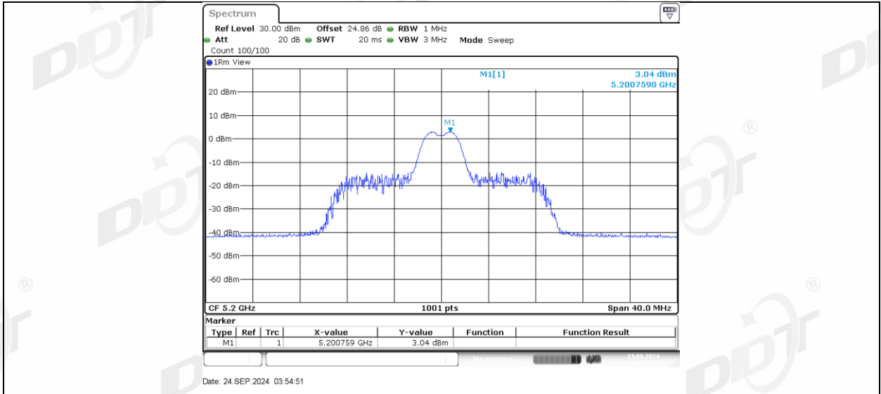
11AX20MIMO Ant2 5200 26Tone RU8
