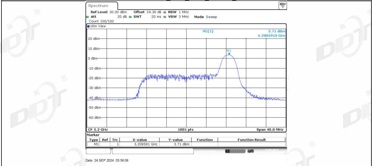
11AX20MIMO Ant2 5200 52Tone RU37
