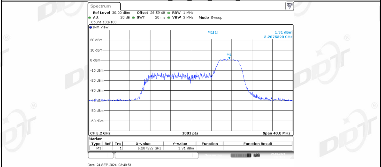
11AX20MIMO Ant1 5200_106Tone RU53
