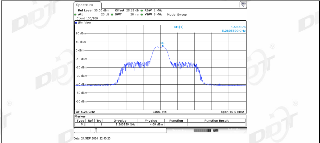
11AX20MIMO Ant1 5260_26Tone RU8
