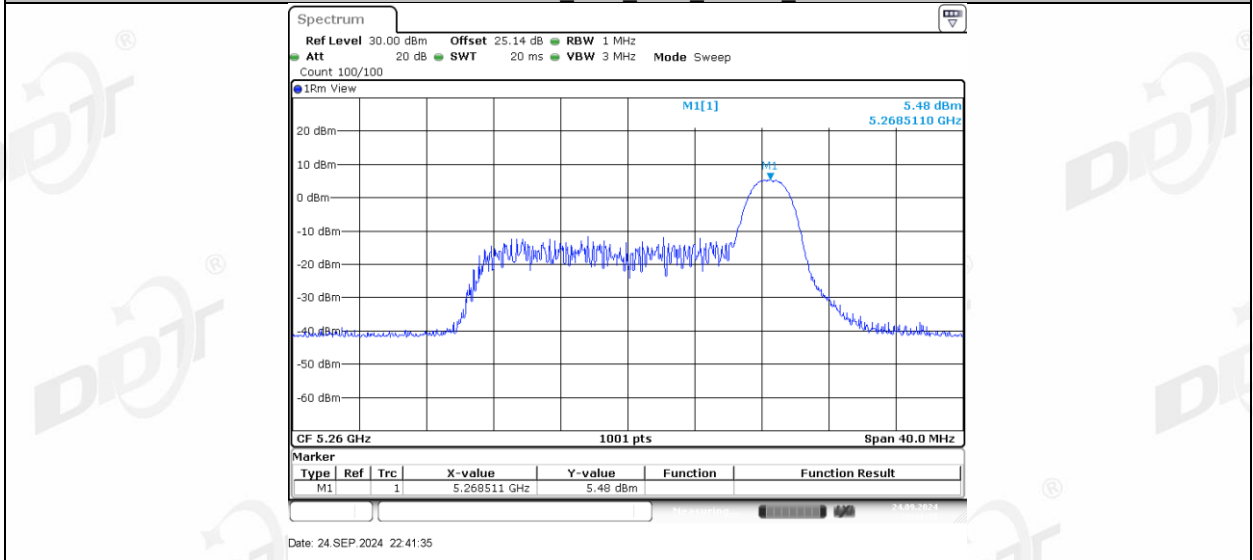
11AX20MIMO Ant1 5260_52Tone RU37
