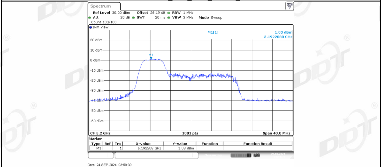
11AX20MIMO Ant2 5200 52Tone RU39
