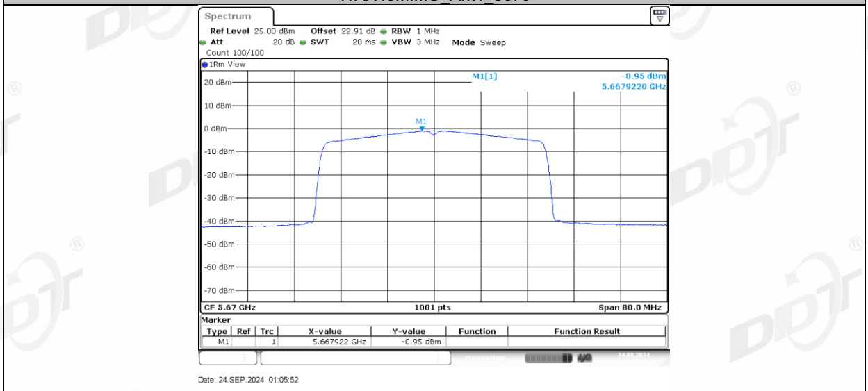
11AX40MIMO Ant2 5670
