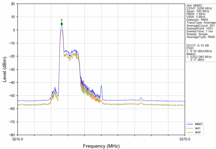
802.11ax(HEW80)_MCH_5290MHz_RU26_Left_MIMO_NTNV
