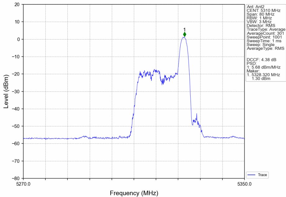
802.11ax(HEW40)_HCH_5310MHz_RU26_Right_Ant2_NTNV
