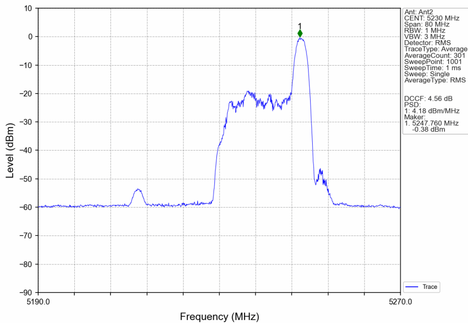
802.11ax(HEW40)_HCH_5230MHz_RU26_Right_Ant2_NTNV
