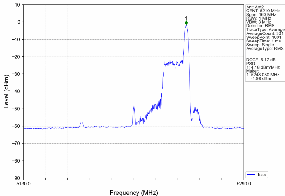
802.11ax(HEW80)_MCH_5210MHz_RU26_Right_MIMO_NTNV
