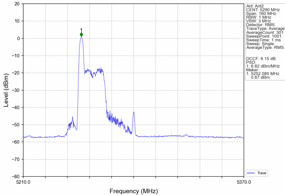
802.11ax(HEW80)_MCH_5290MHz_RU26_Left_MIMO_NTNV
