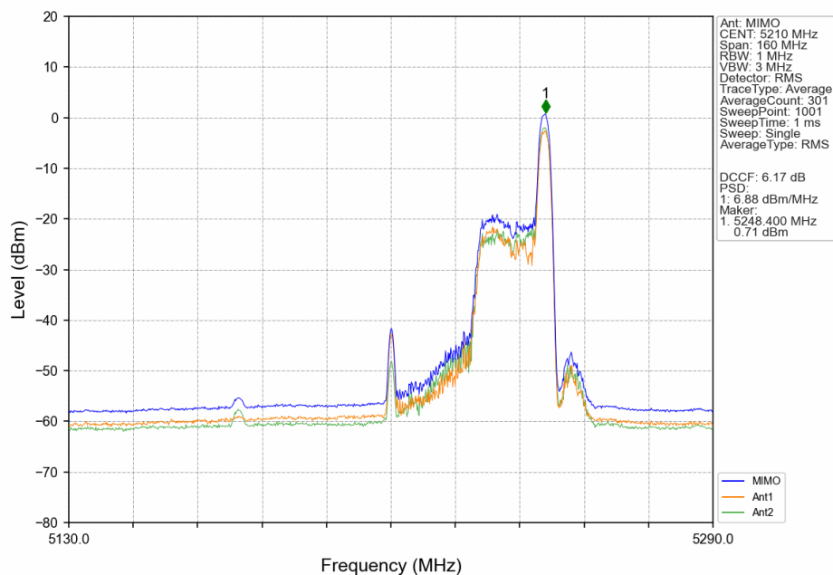
802.11ax(HEW80)_MCH_5210MHz_RU26_Right_MIMO_NTNV
