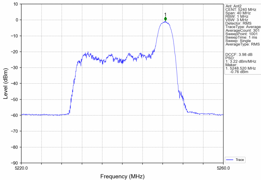
802.11ax(HEW20)_HCH_5240MHz_RU26_Right_Ant2_NTNV
