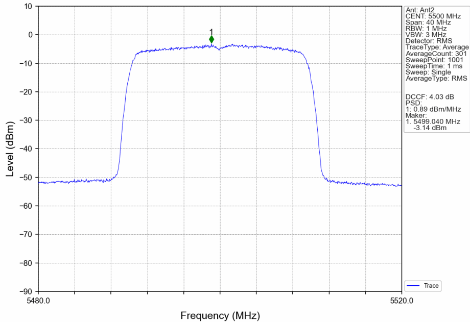
802.11ax(HEW20)_LCH_5500MHz_RU242_Left_MIMO_NTNV
