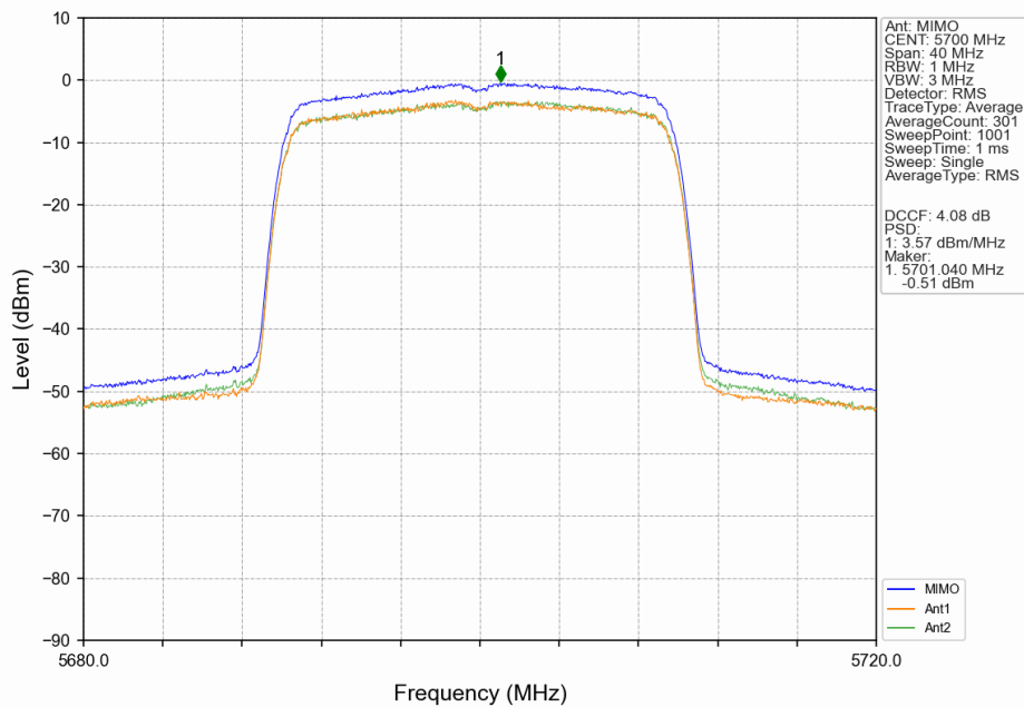
802.11ax(HEW20)_HCH_5700MHz_RU242_Left_MIMO_NTNV
