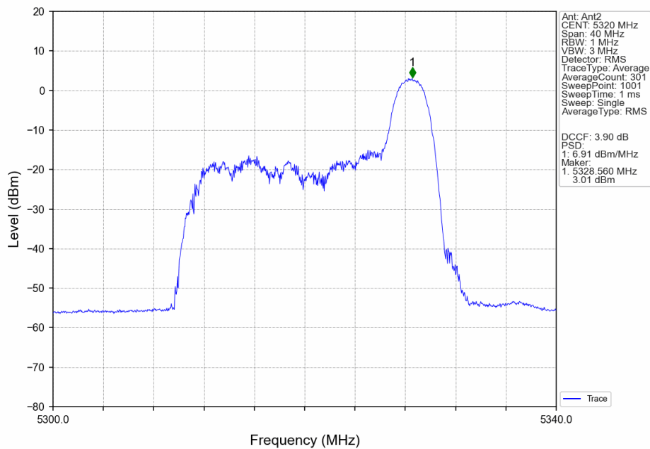
802.11ax(HEW20)_HCH_5320MHz_RU26_Right_Ant2_NTNV
