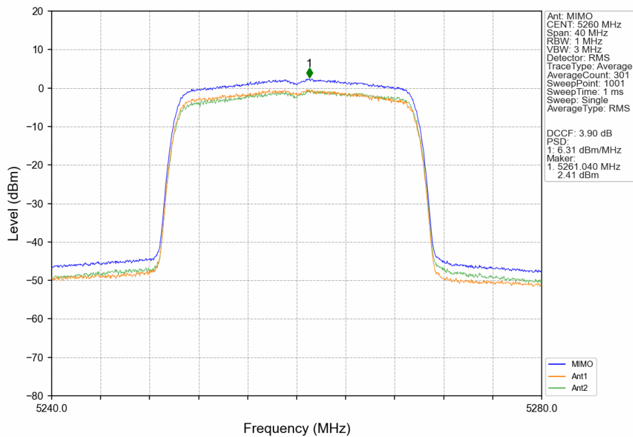
802.11ax(HEW20)_LCH_5260MHz_RU242_Left_MIMO_NTNV
