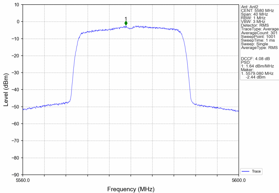
802.11ax(HEW20)_MCH_5580MHz_RU242_Left_MIMO_NTNV
