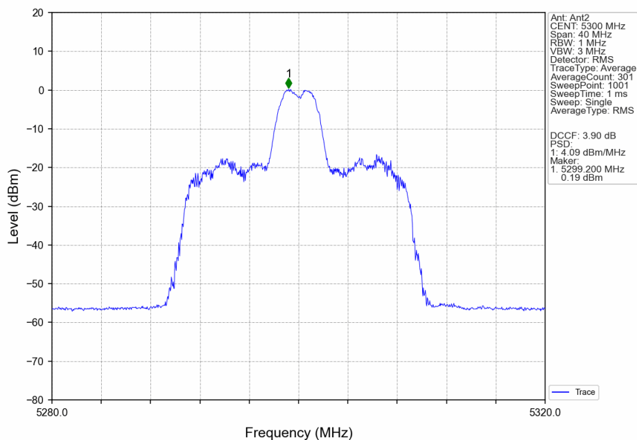
802.11ax(HEW20)_MCH_5300MHz_RU26_Mid_Ant2_NTNV
