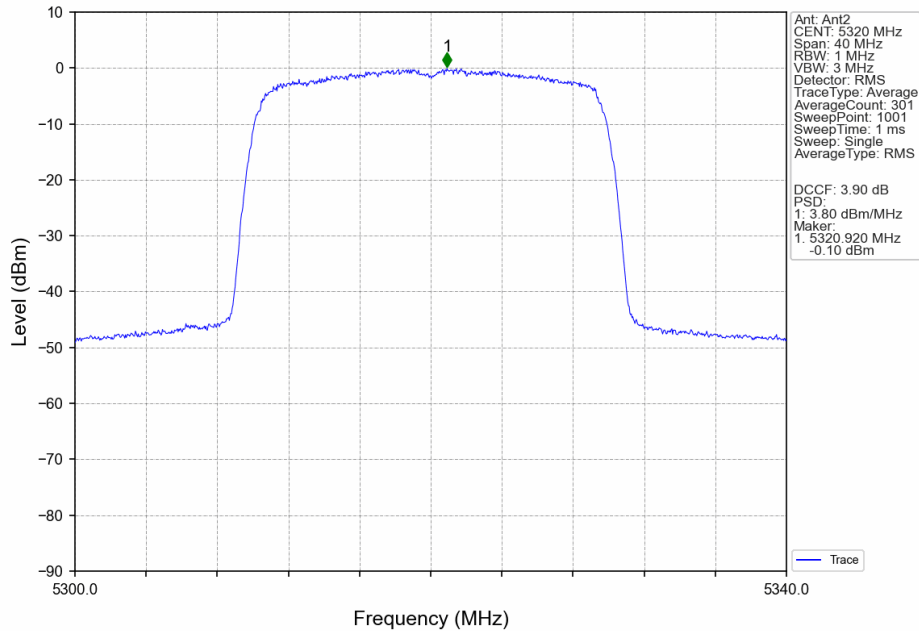
802.11ax(HEW20)_HCH_5320MHz_RU242_Left_MIMO_NTNV
