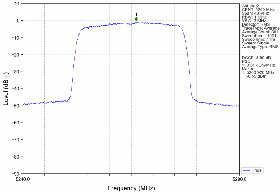
802.11ax(HEW20)_LCH_5260MHz_RU242_Left_MIMO_NTNV
