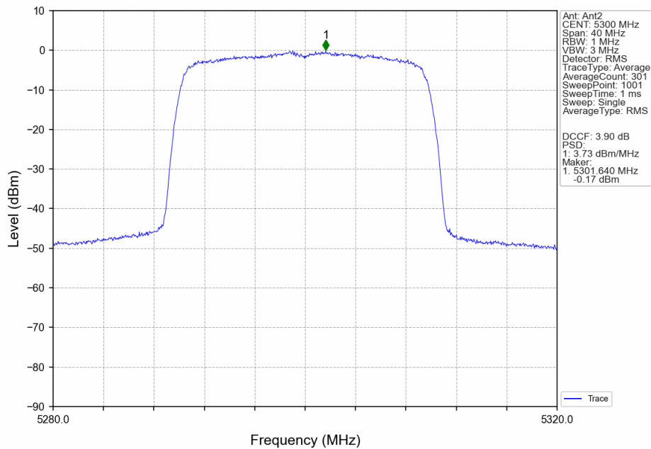
802.11ax(HEW20)_MCH_5300MHz_RU242_Left_MIMO_NTNV
