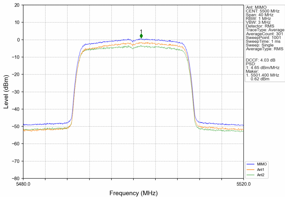
802.11ax(HEW20)_LCH_5500MHz_RU242_Left_MIMO_NTNV
