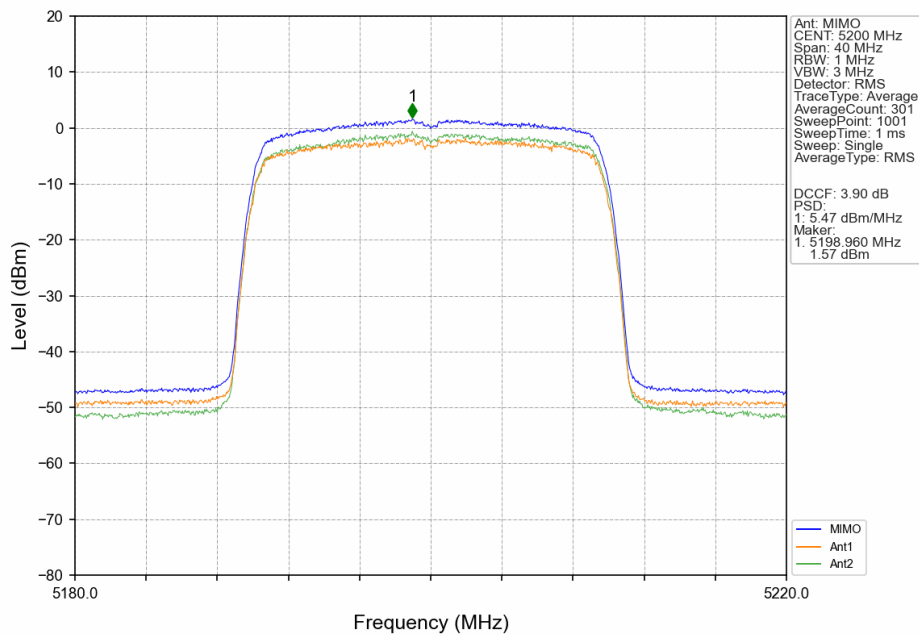
802.11ax(HEW20)_MCH_5200MHz_RU242_Left_MIMO_NTNV
