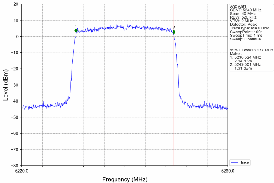
802.11ax(HEW20)_HCH_5240MHz_RU242_Left_Ant1_NTNV
