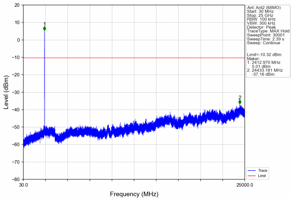
802.11ax(HEW20)_LCH_2412MHz_RU26_Mid_Ant2 (MIMO)_NTNV
