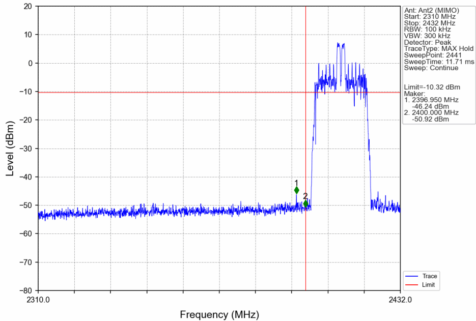
802.11ax(HEW20)_LCH_2412MHz_RU26_Mid_Ant2 (MIMO)_NTNV
