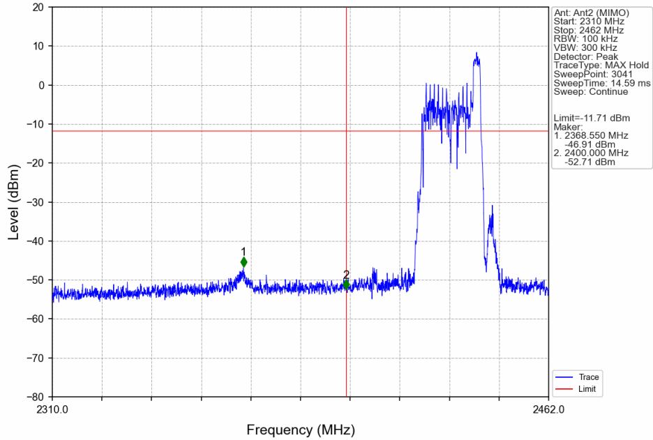
802.11ax(HEW40)_LCH_2422MHz_RU26_Right_Ant2 (MIMO)_NTNV
