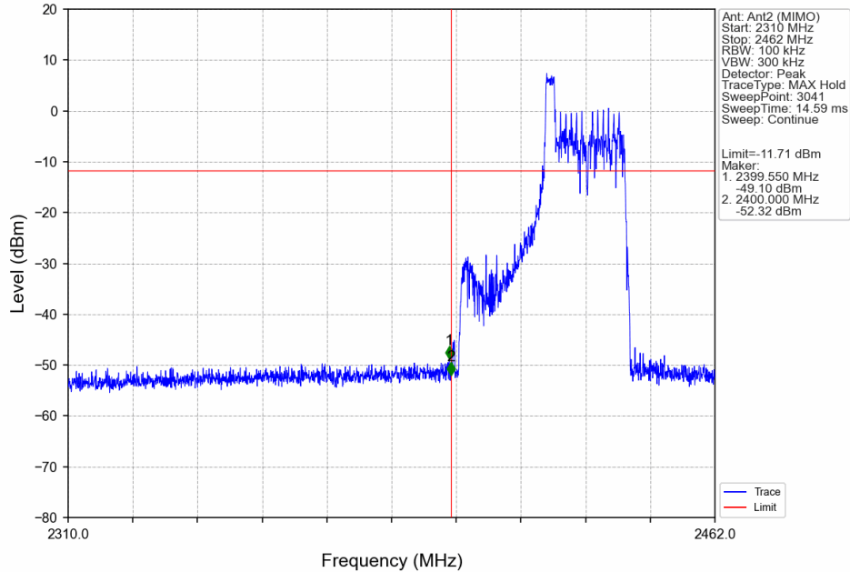
802.11ax(HEW40)_LCH_2422MHz_RU26_Mid_Ant2 (MIMO)_NTNV
