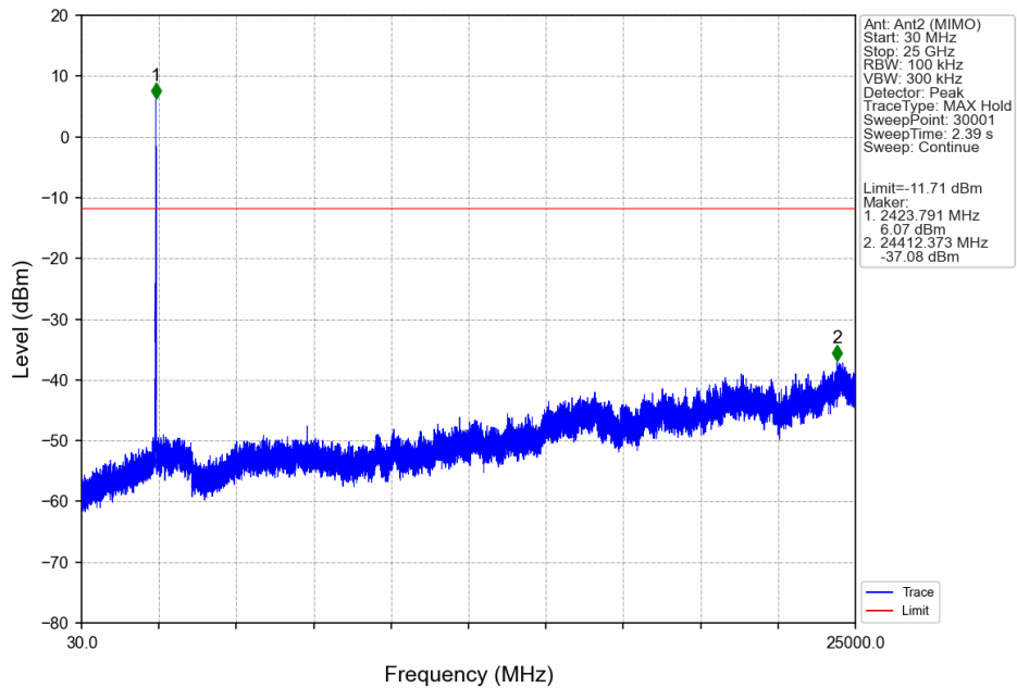
802.11ax(HEW40)_LCH_2422MHz_RU26_Mid_Ant2 (MIMO)_NTNV
