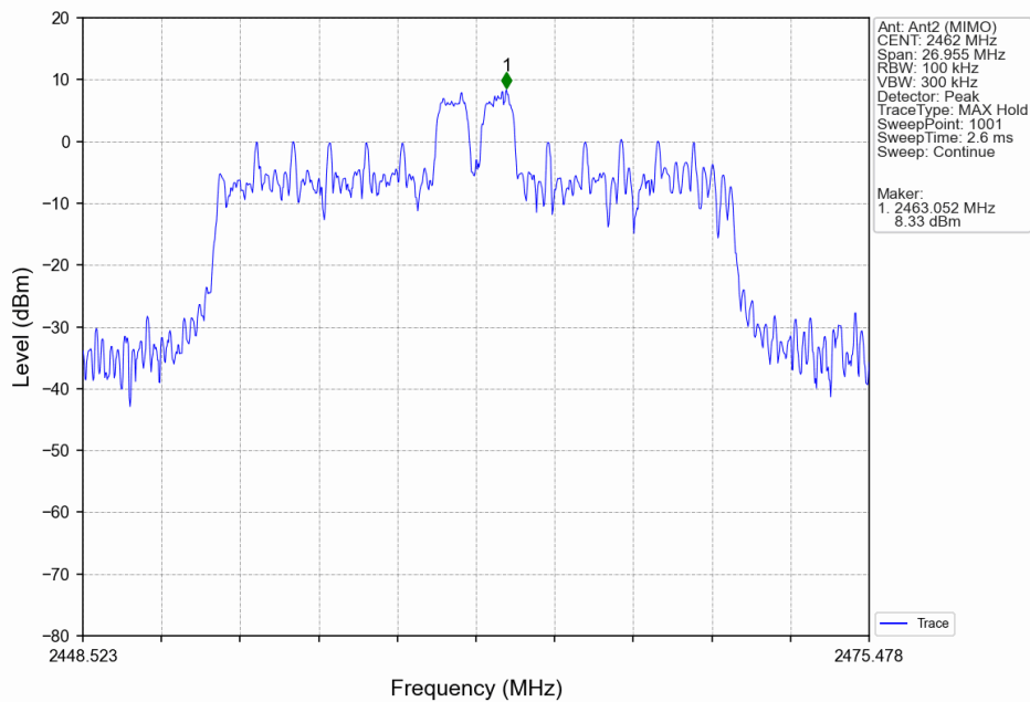
802.11ax(HEW20)_HCH_2462MHz_RU26_Mid_Ant2 (MIMO)_NTNV
