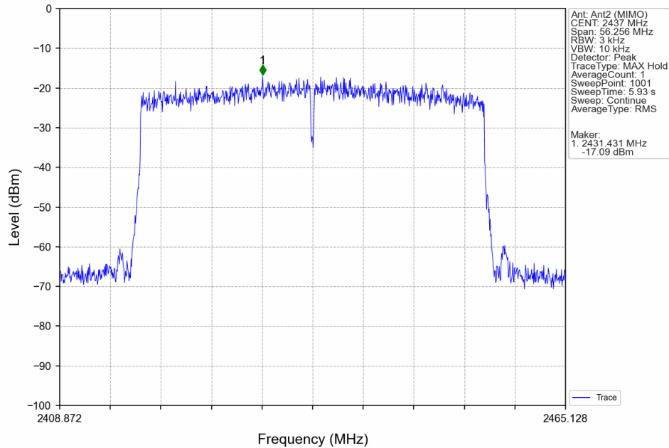
802.11ax(HEW40)_MCH_2437MHz_RU484_Left_MIMO_NTNV
