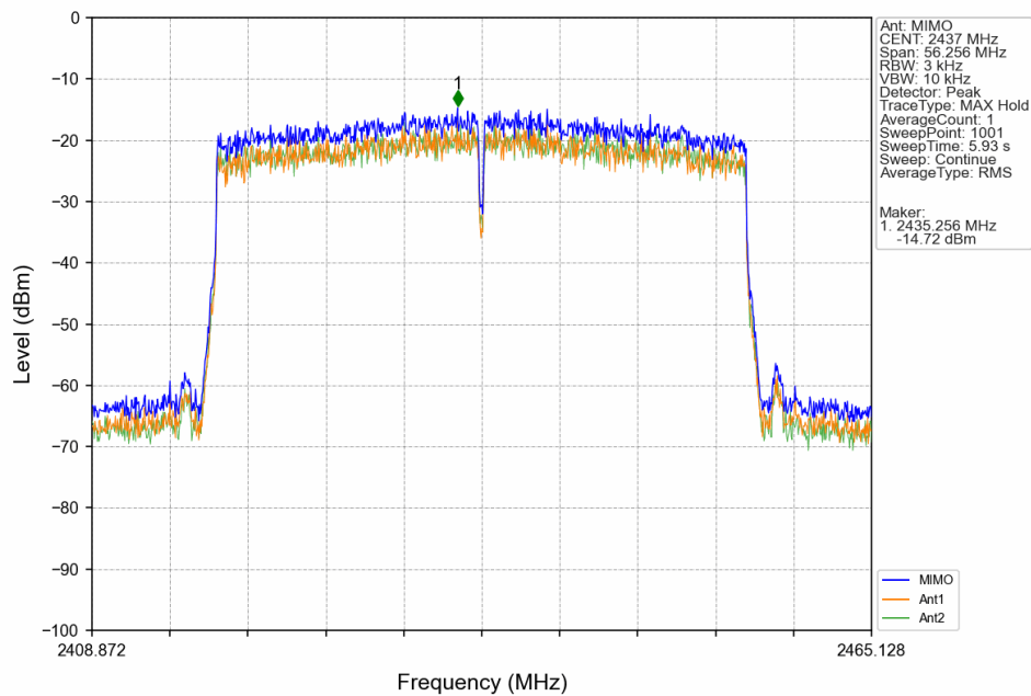
802.11ax(HEW40)_MCH_2437MHz_RU484_Left_MIMO_NTNV
