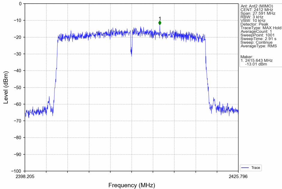
802.11ax(HEW20)_LCH_2412MHz_RU242_Left_MIMO_NTNV
