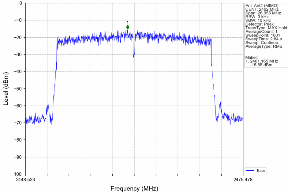
802.11ax(HEW20)_HCH_2462MHz_RU242_Left_MIMO_NTNV
