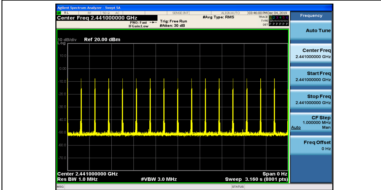
Dwell Time_DH5_2441
