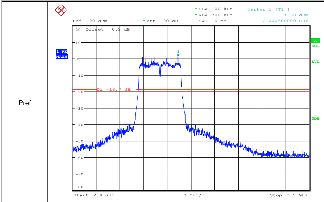
RF Conducted Spurious Emissions_11N20SISO_2437 ant2
