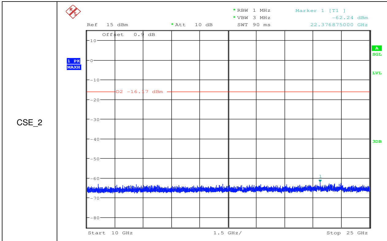
RF Conducted Spurious Emissions_11B_2462 ant2
