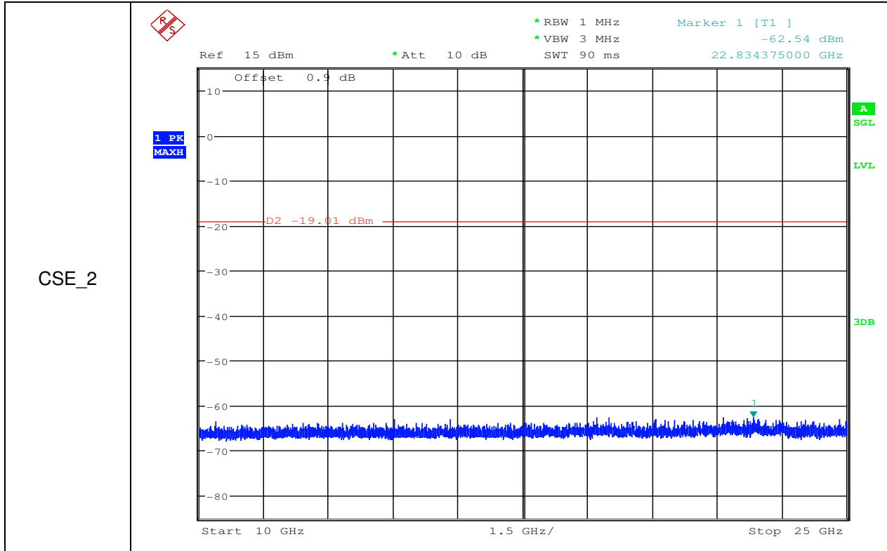
RF Conducted Spurious Emissions_11G_2437 ant2
