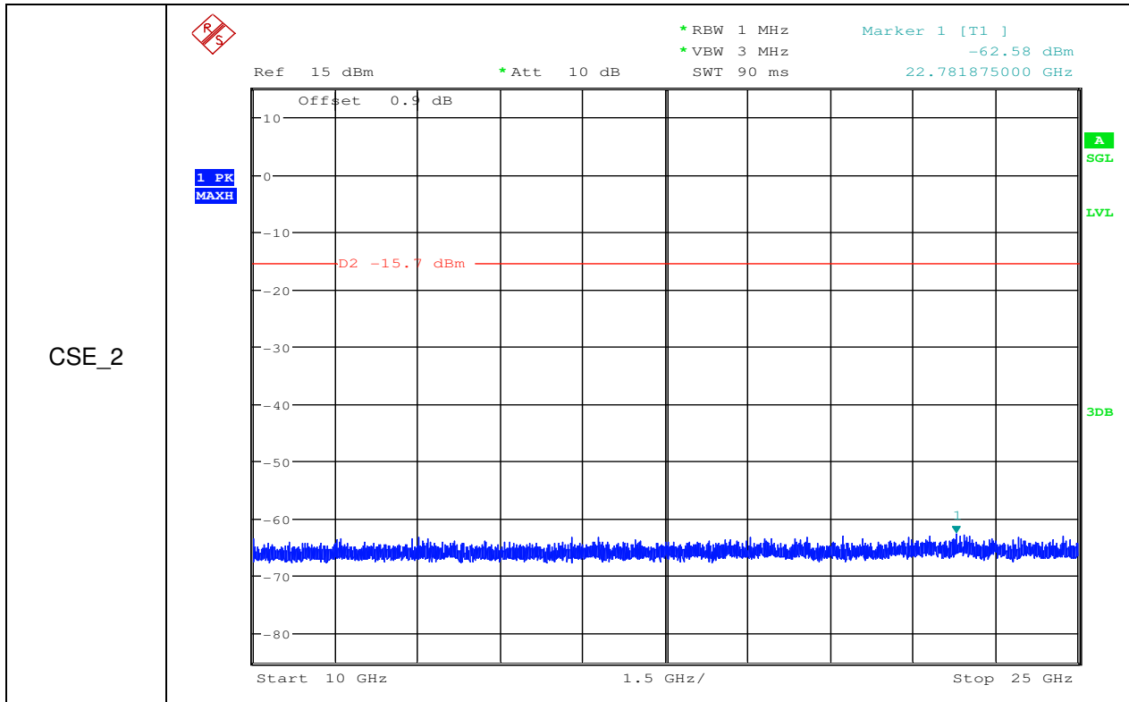
RF Conducted Spurious Emissions_11B_2412 ant2
