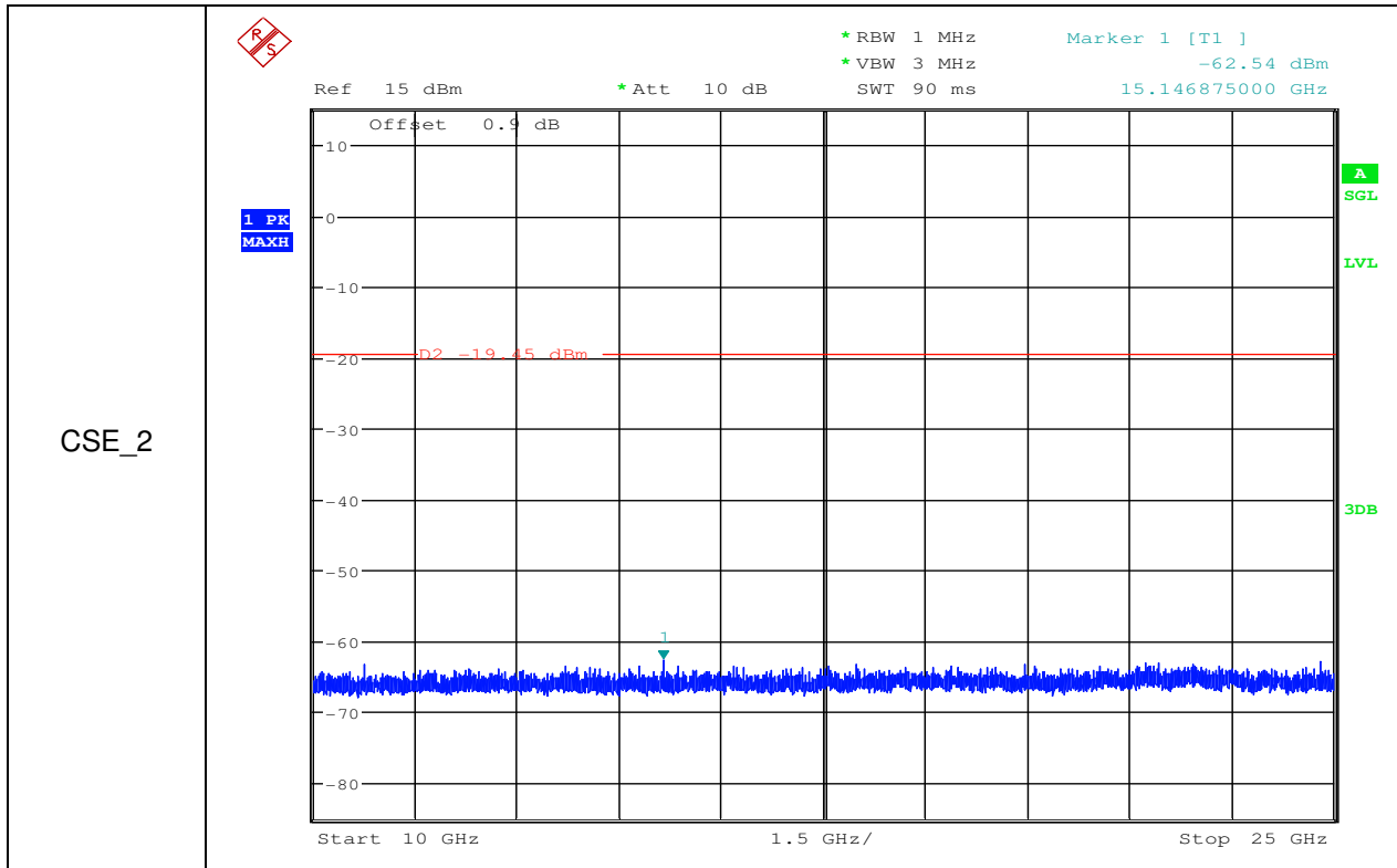
RF Conducted Spurious Emissions_11G_2412 ant2
