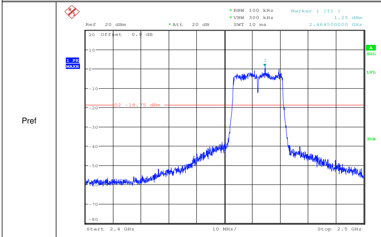
RF Conducted Spurious Emissions_11N20SISO_2462 ant2
