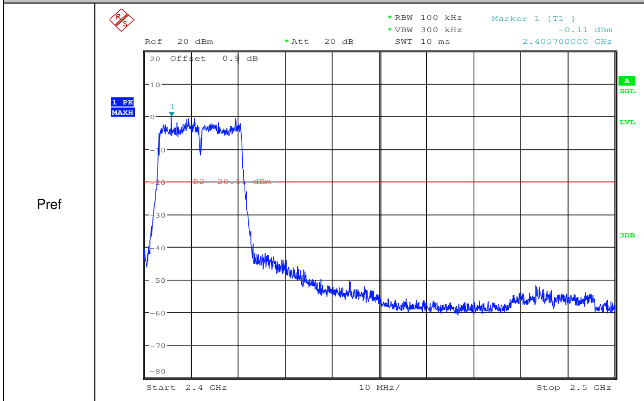
RF Conducted Spurious Emissions_11N20SISO_2412 ant2
