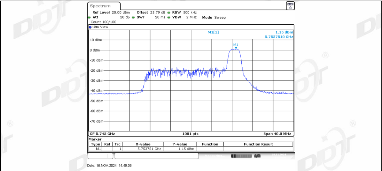
11AX20MIMO Ant2 5745_52Tone RU37
