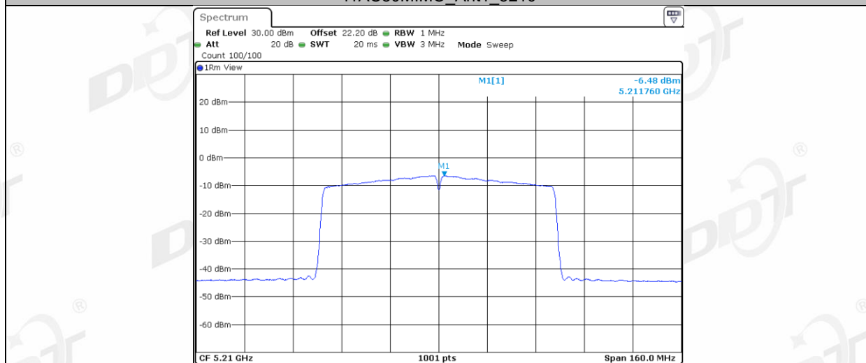
11AC80MIMO Ant2 5210
