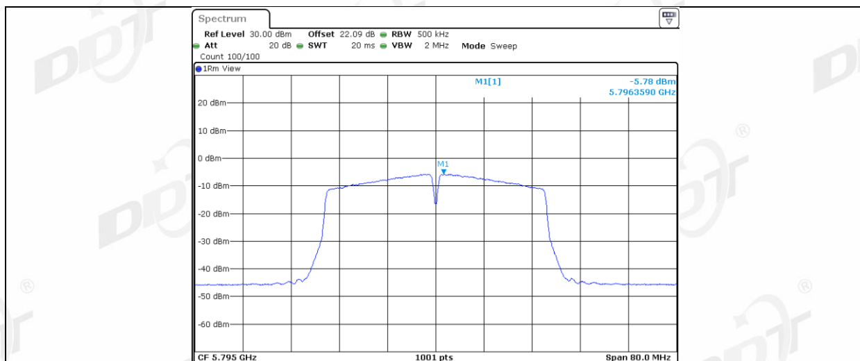
11AC40MIMO Ant2 5795
