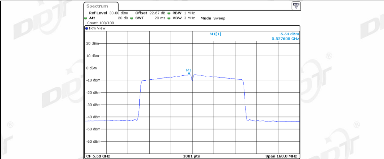
11AC80MIMO Ant2 5530
