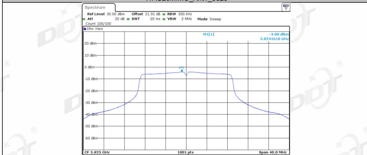
11AC20MIMO Ant2 5825
