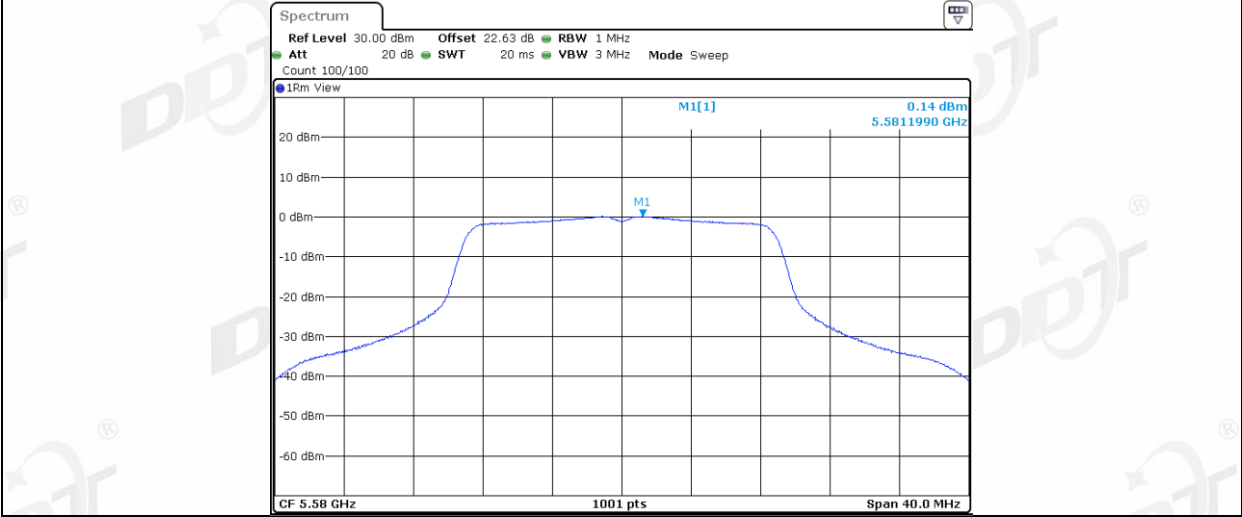
11AC20MIMO Ant2 5580
