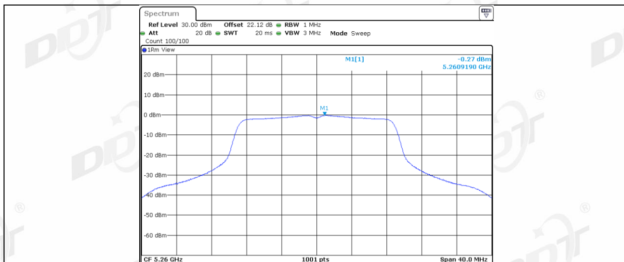
11AC20MIMO Ant2 5260
