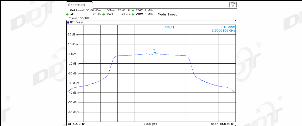
11AC20MIMO Ant2 5500
