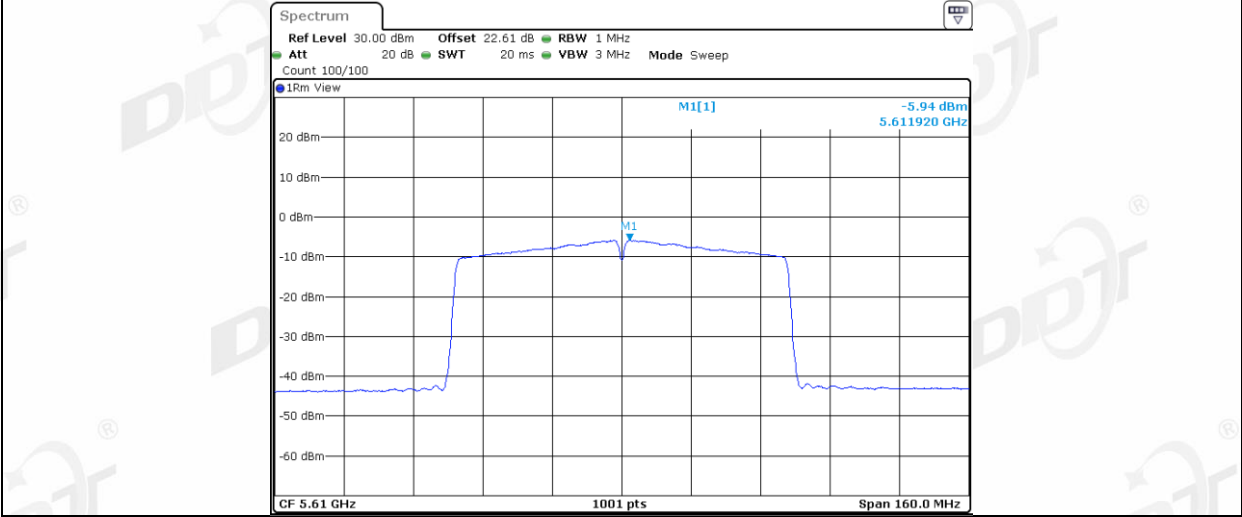
11AC80MIMO Ant2 5610
