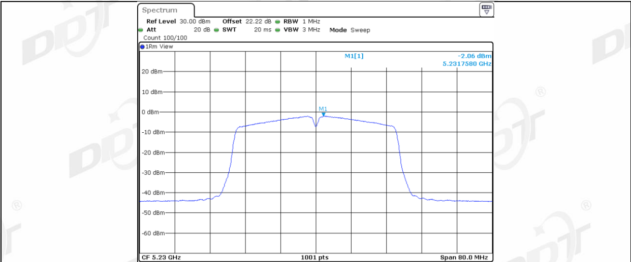
11AC40MIMO Ant2 5230
