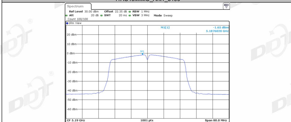
11AC40MIMO Ant2 5190
