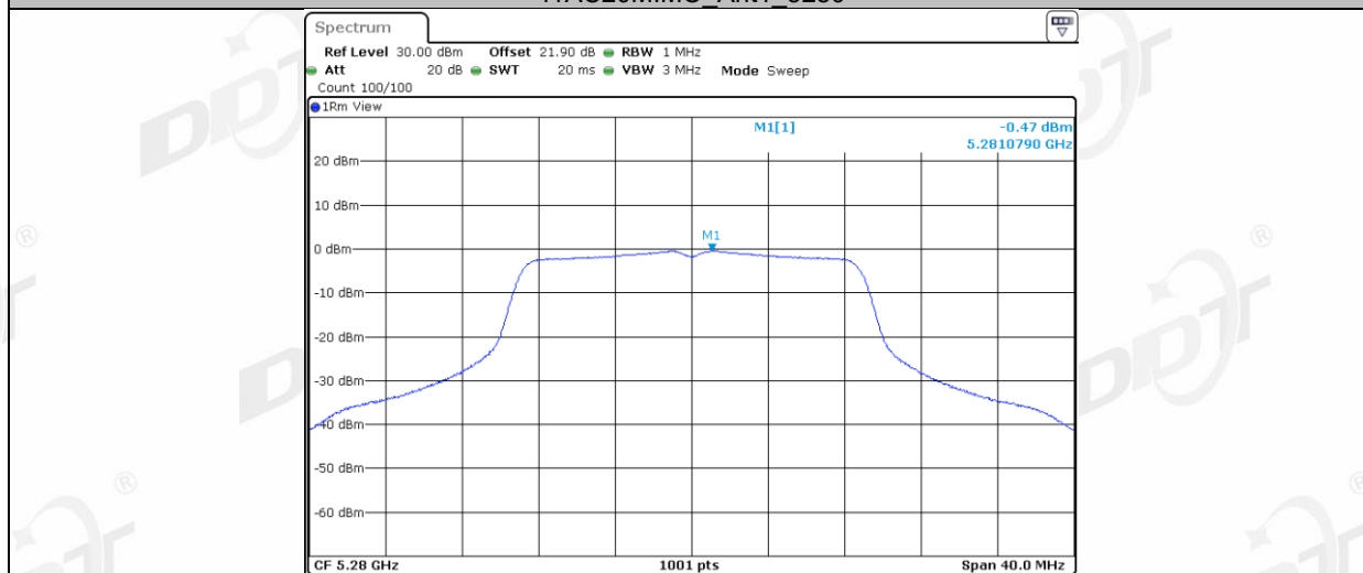
11AC20MIMO Ant2 5280
