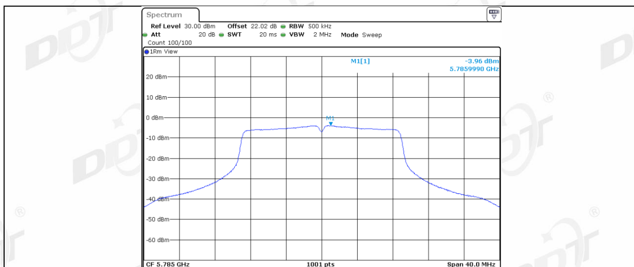
11AC20MIMO Ant2 5785
