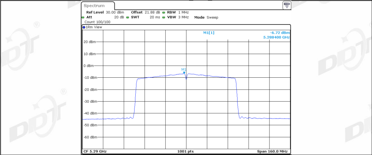
11AC80MIMO Ant2 5290
