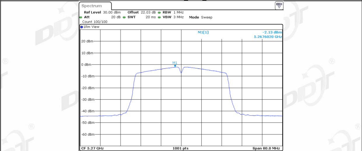
11AC40MIMO Ant2 5270
