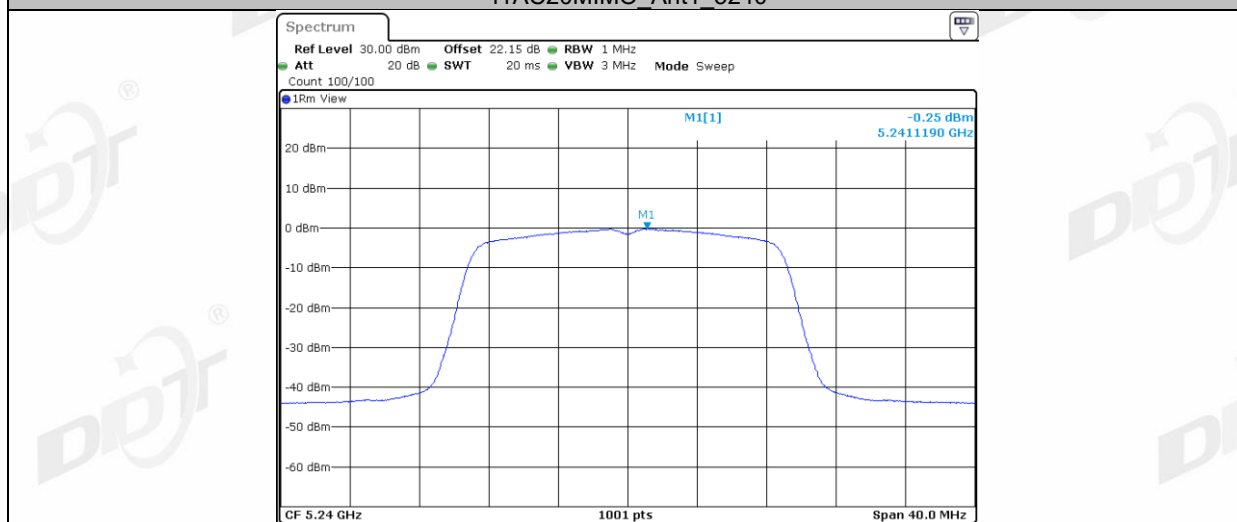
11AC20MIMO Ant2 5240
