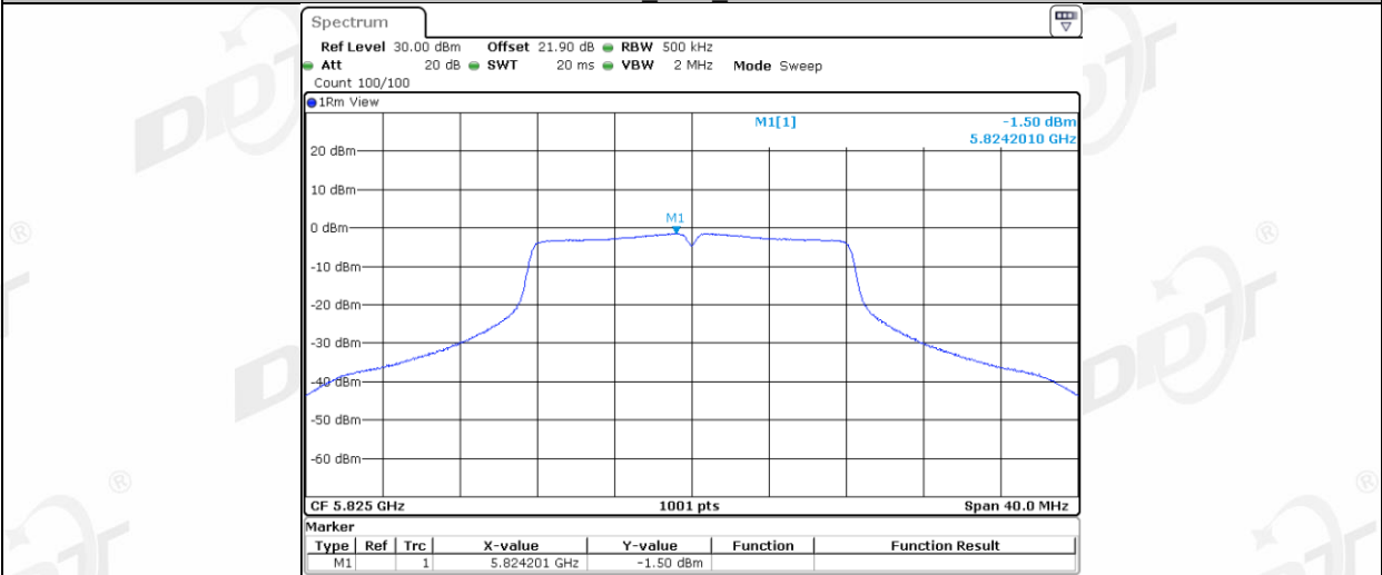
11A Ant2 5825
