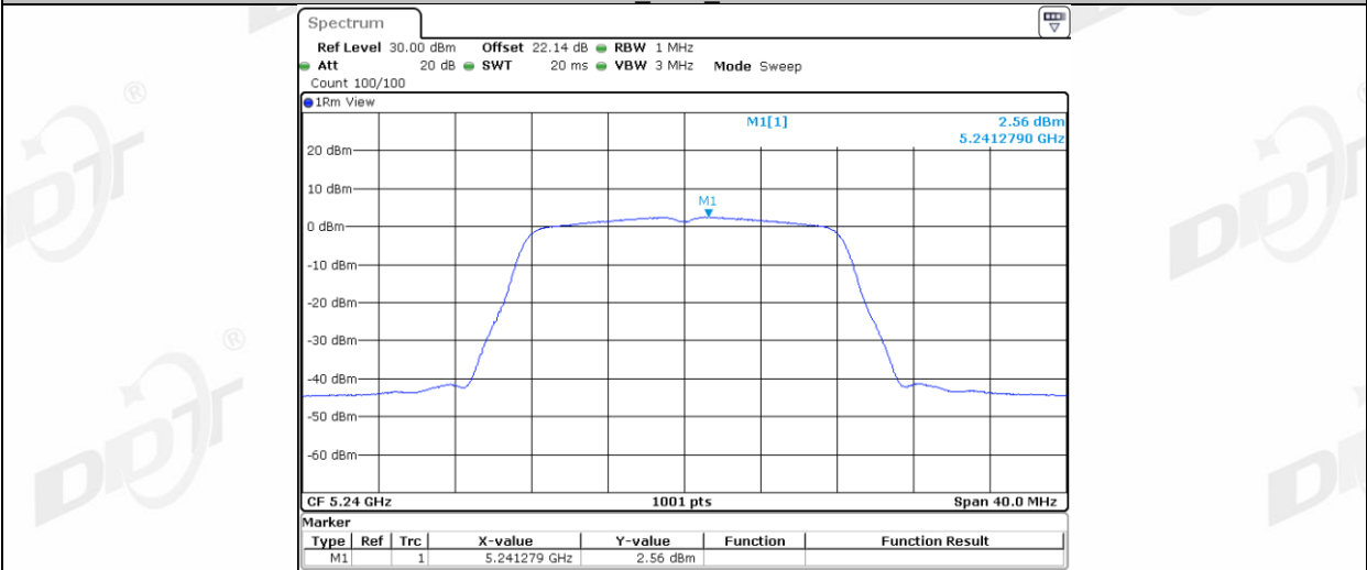
11A Ant2 5240
