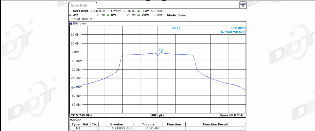
11A Ant2_5745
