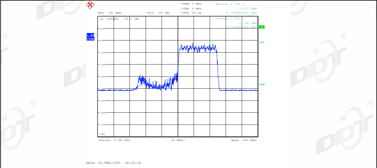
11AX80MIMO Ant2 5690 UNII-2C 484Tone RU65
