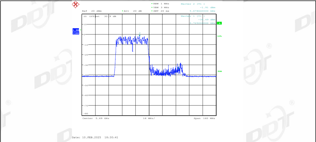
11AX80MIMO Ant2 5690 UNII-2C 484Tone RU66
