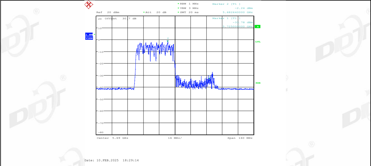
11AX80MIMO Ant1 5690 UNII-2C 484Tone RU66
