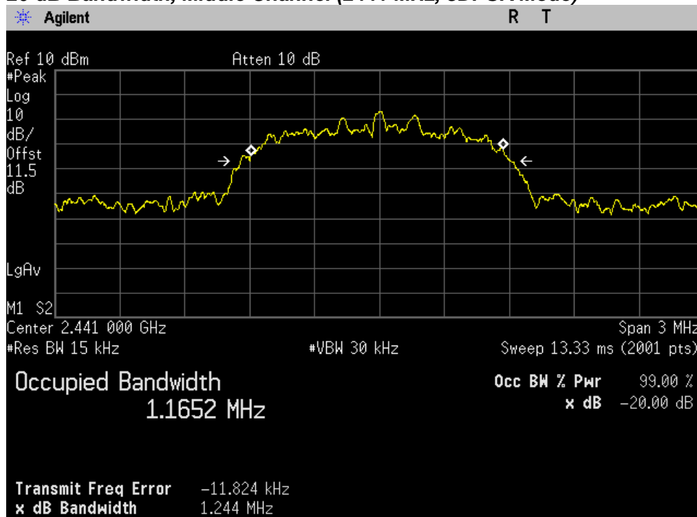
20 dB Bandwidth, Middle Channel (2441 MHz, 8DPSK Mode)
