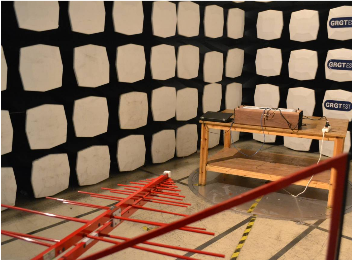
RSE (Above 1GHz)
