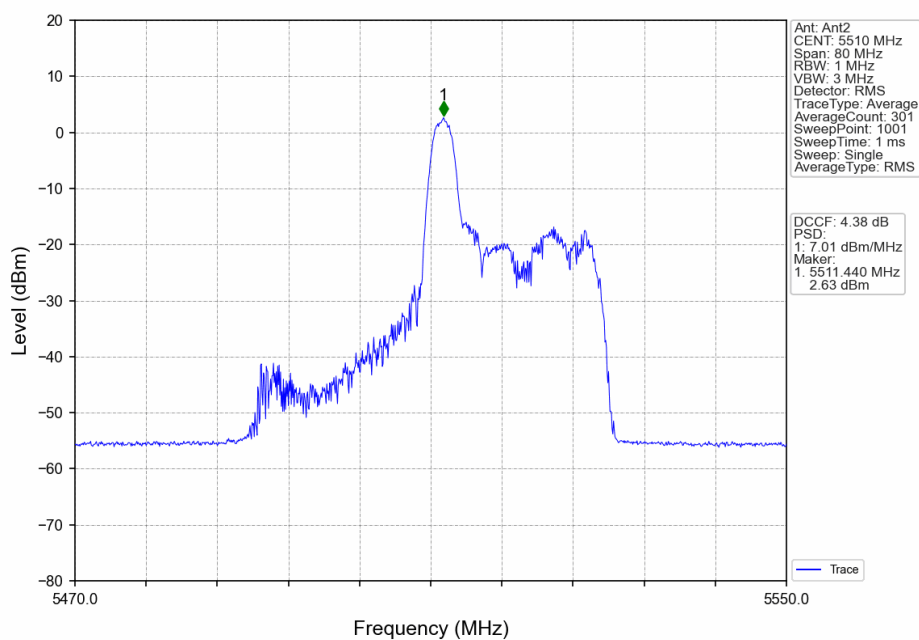
802.11ax(HEW40)_LCH_5510MHz_RU26_Mid_Ant2_NTNV
