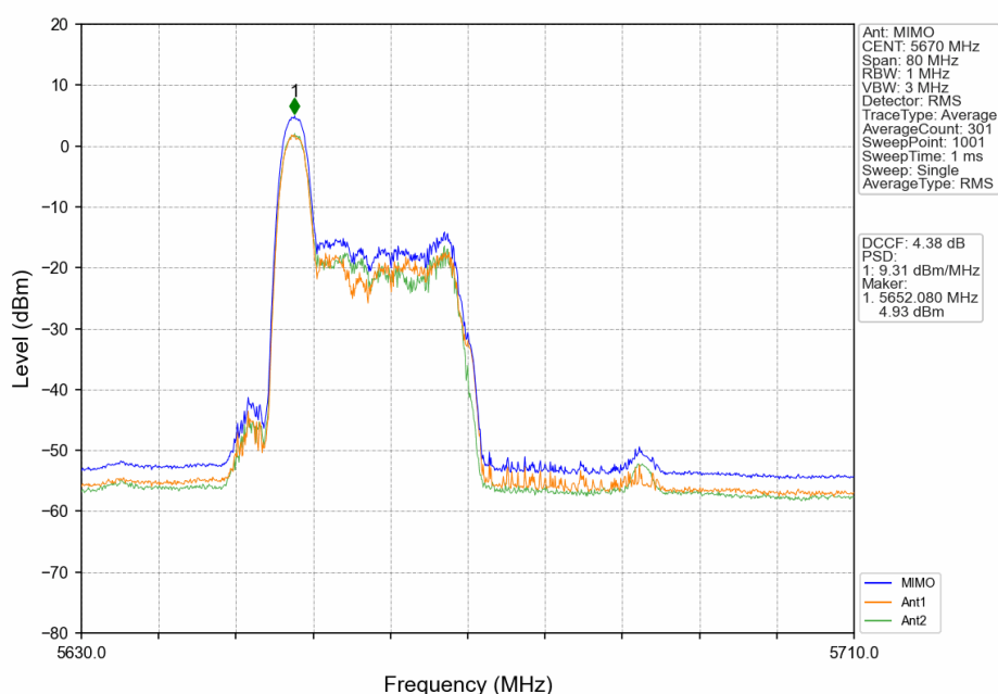
802.11ax(HEW40)_HCH_5670MHz_RU26_Left_MIMO_NTNV
