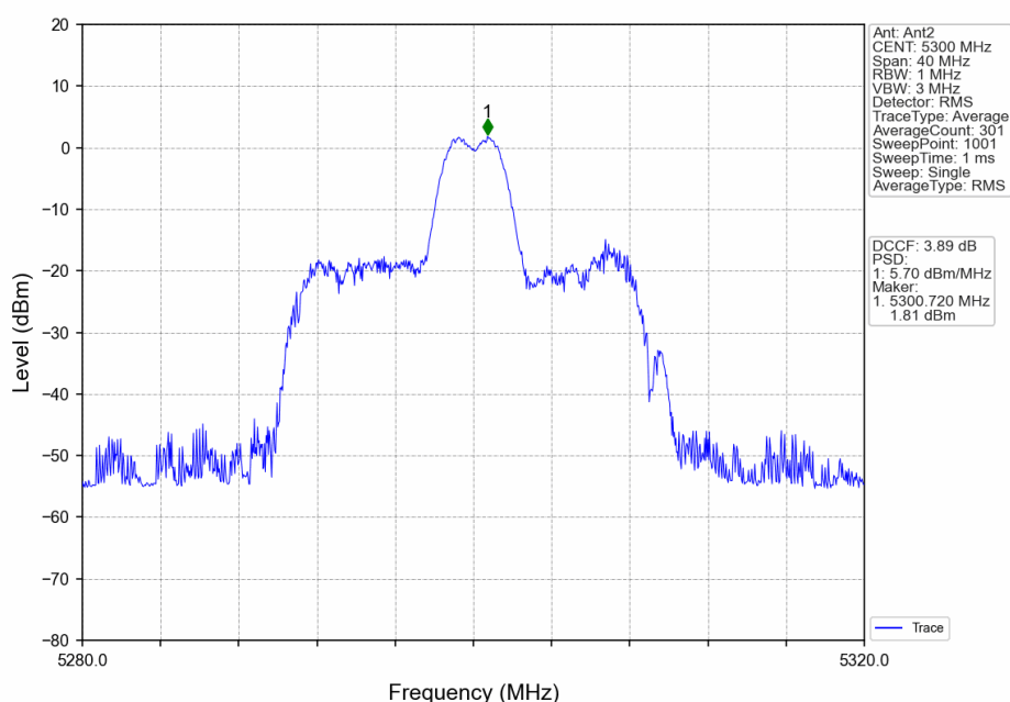
802.11ax(HEW20)_MCH_5300MHz_RU26_Mid_Ant2_NTNV
