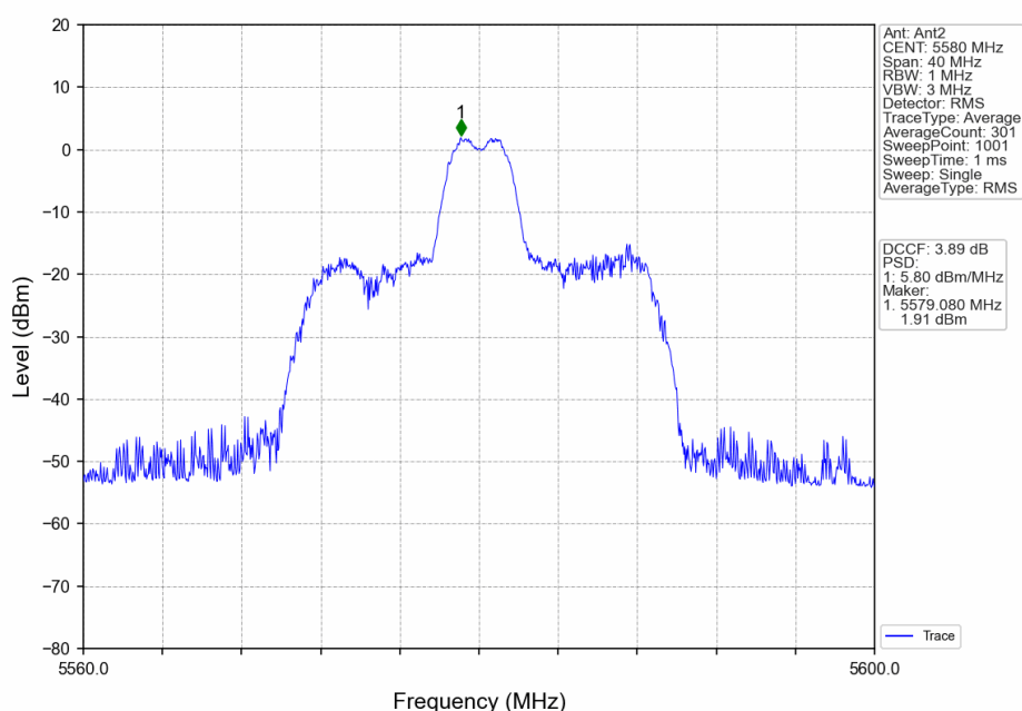
802.11ax(HEW20)_MCH_5580MHz_RU26_Mid_Ant2_NTNV
