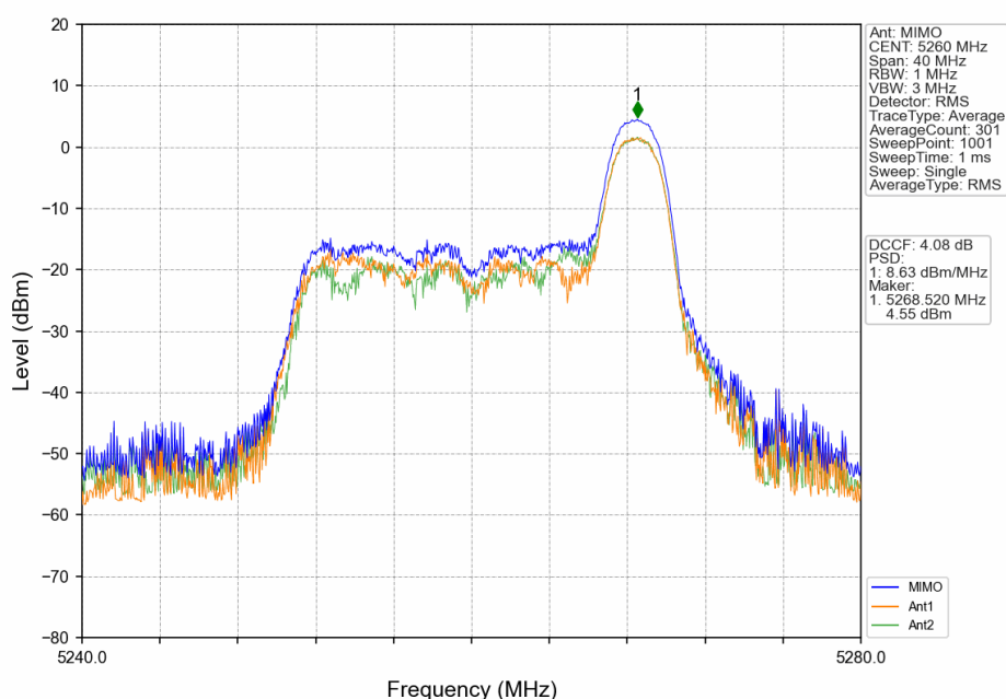
802.11ax(HEW20)_LCH_5260MHz_RU26_Right_MIMO_NTNV
