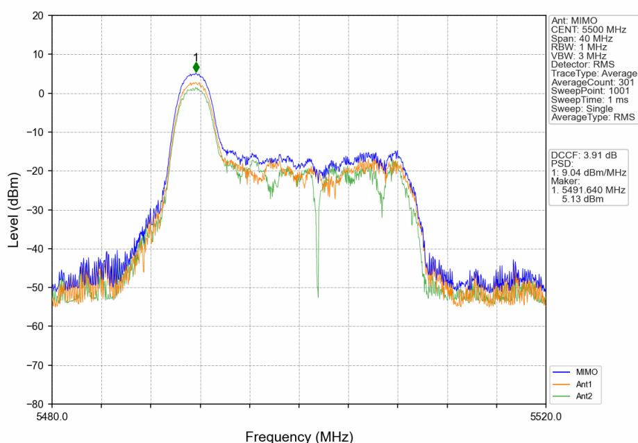
802.11ax(HEW20)_LCH_5500MHz_RU26_Left_MIMO_NTNV
