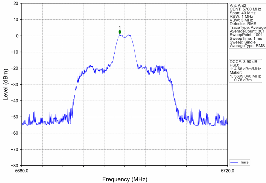
802.11ax(HEW20)_HCH_5700MHz_RU26_Right_MIMO_NTNV
