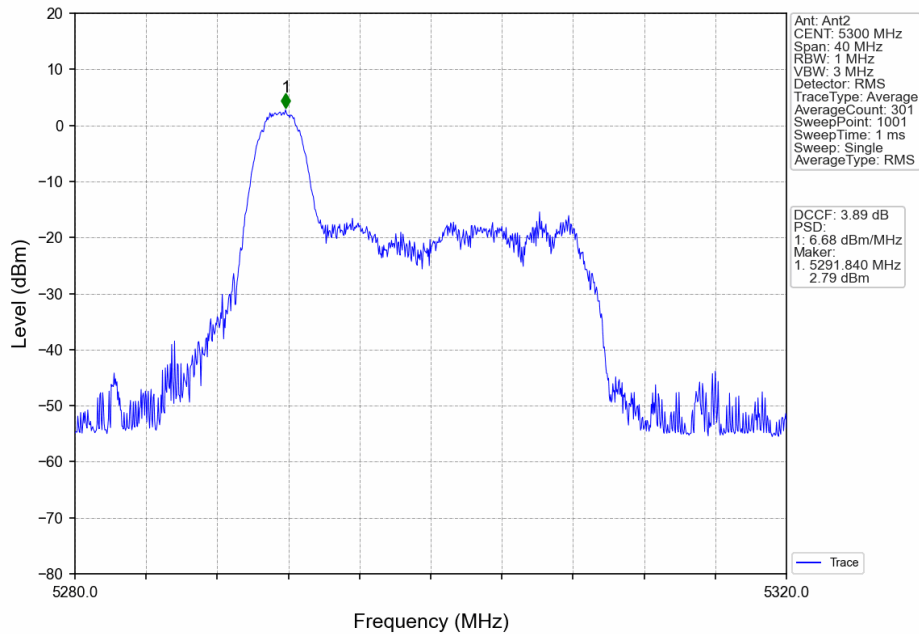
802.11ax(HEW20)_MCH_5300MHz_RU26_Left_MIMO_NTNV
