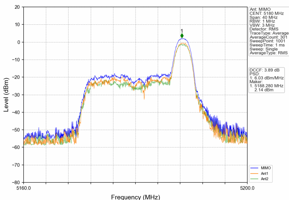
802.11ax(HEW20)_LCH_5180MHz_RU26_Right_MIMO_NTNV
