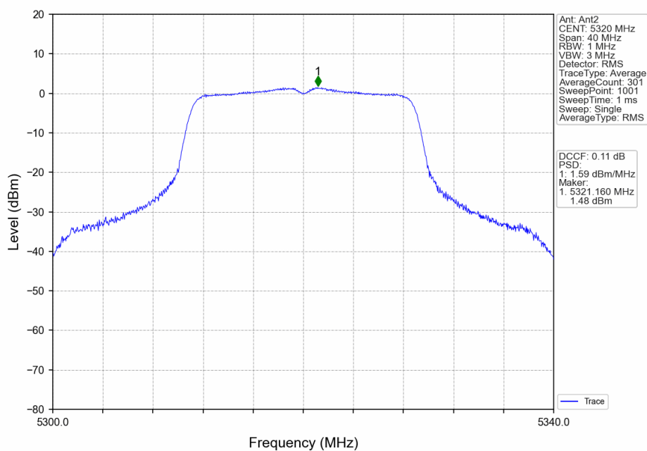
802.11ac(VHT20)_HCH_5320MHz_Ant2_NTNV
