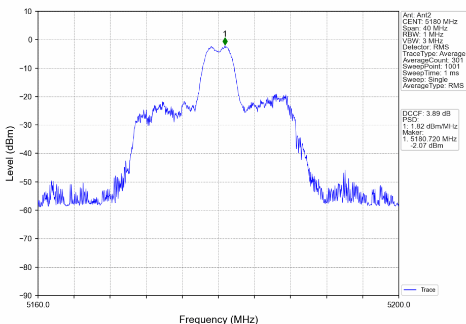
802.11ax(HEW20)_LCH_5180MHz_RU26_Mid_Ant2_NTNV
