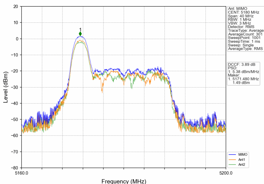
802.11ax(HEW20)_LCH_5180MHz_RU26_Left_MIMO_NTNV
