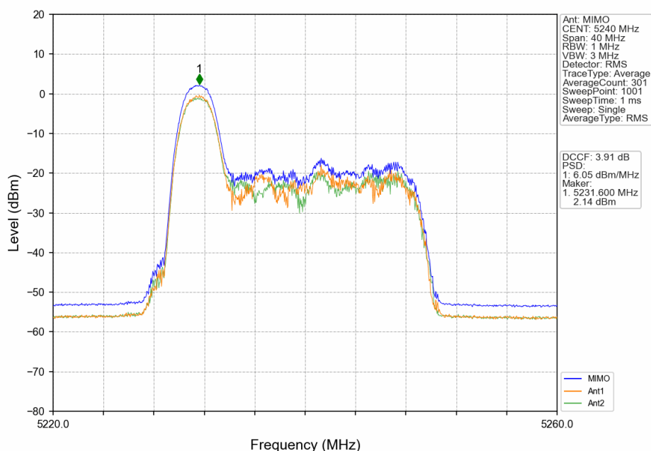
802.11ax(HEW20)_HCH_5240MHz_RU26_Left_MIMO_NTNV
