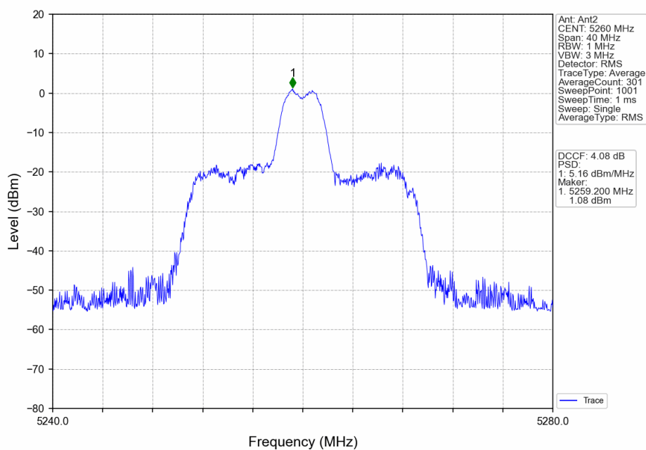
802.11ax(HEW20)_LCH_5260MHz_RU26_Mid_Ant2_NTNV
