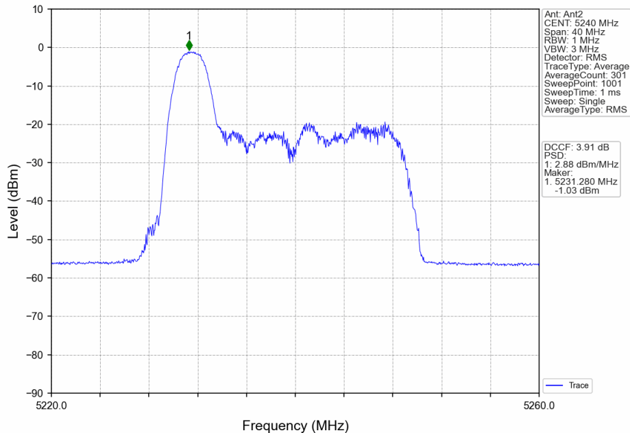
802.11ax(HEW20)_HCH_5240MHz_RU26_Left_MIMO_NTNV
