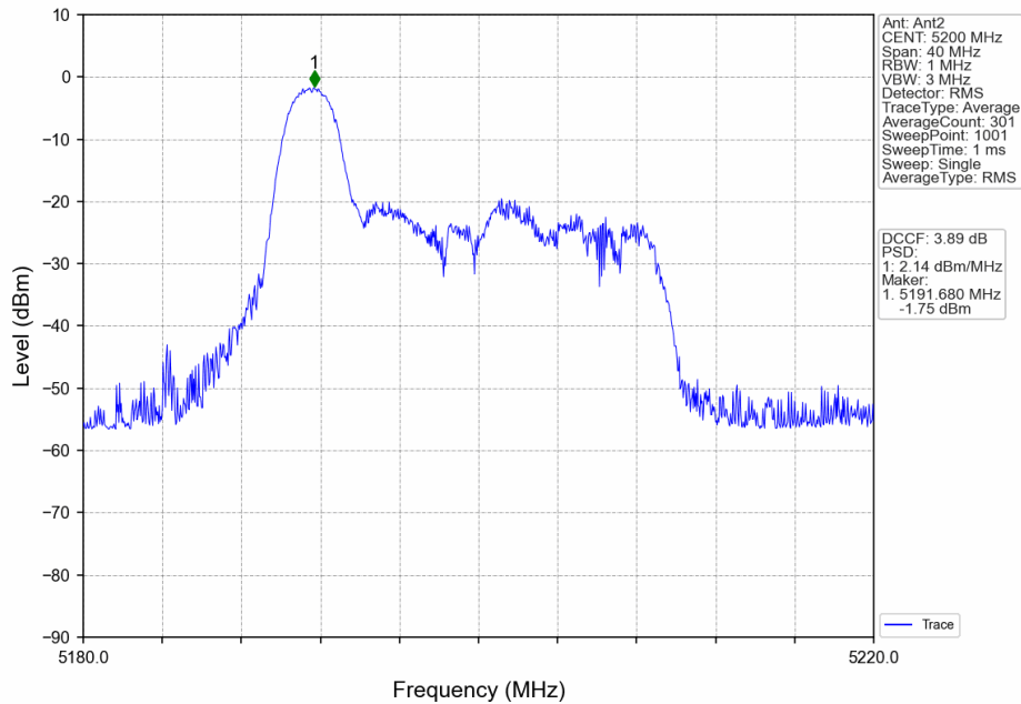
802.11ax(HEW20)_MCH_5200MHz_RU26_Left_MIMO_NTNV
