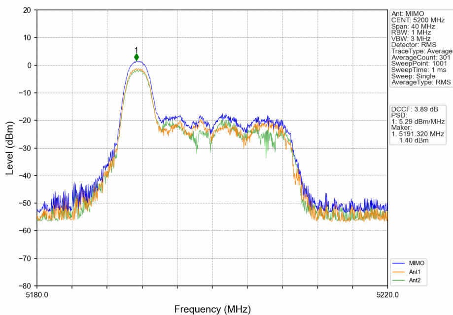
802.11ax(HEW20)_MCH_5200MHz_RU26_Left_MIMO_NTNV
