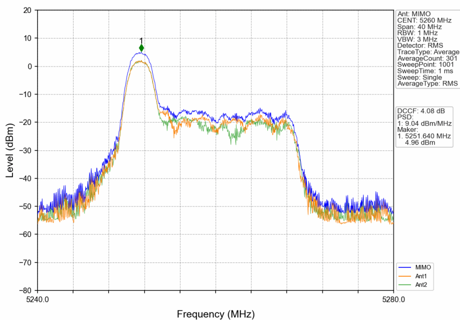
802.11ax(HEW20)_LCH_5260MHz_RU26_Left_MIMO_NTNV
