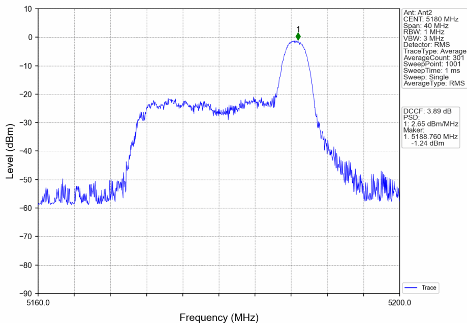
802.11ax(HEW20)_LCH_5180MHz_RU26_Right_MIMO_NTNV
