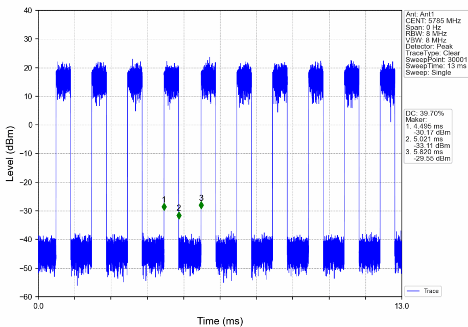
802.11ax(HEW20)_MCH_5785MHz_RU242_Left_Ant1_NTNV
