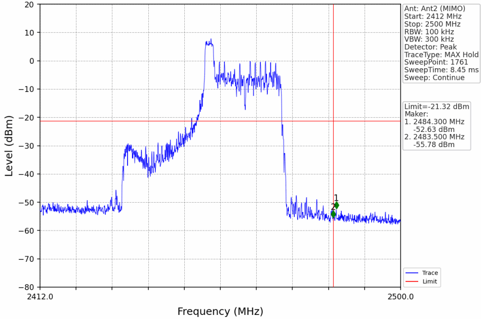
802.11ax(HEW40)_HCH_2452MHz_RU26_Mid_Ant2 (MIMO)_NTNV
