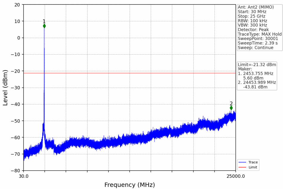
802.11ax(HEW40)_HCH_2452MHz_RU26_Mid_Ant2 (MIMO)_NTNV
