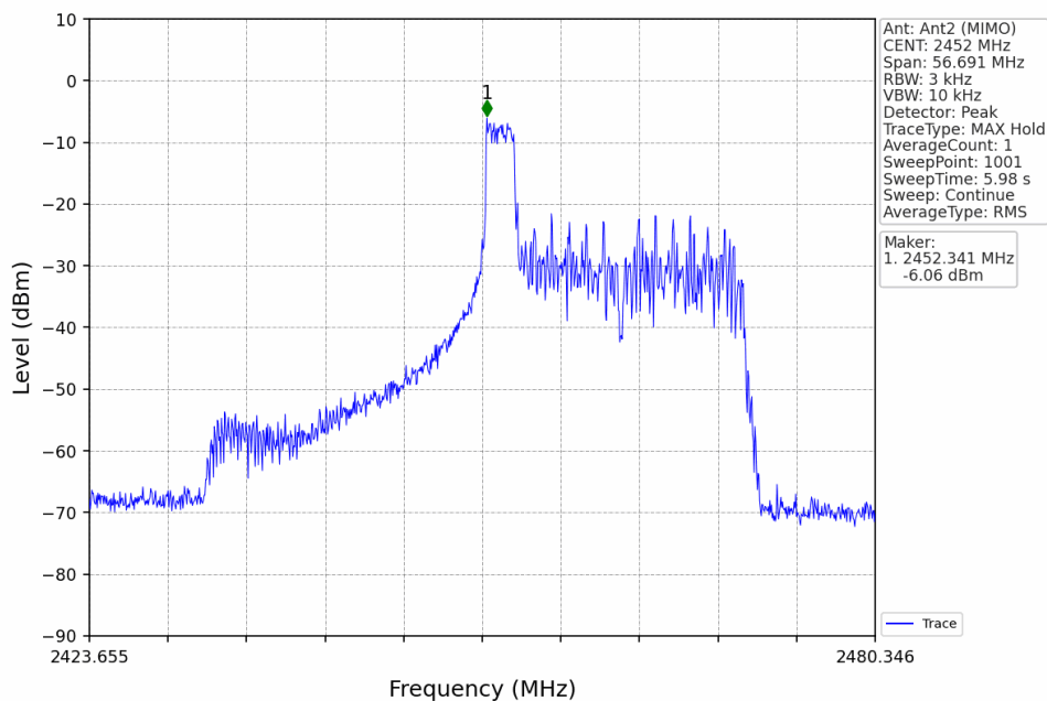
802.11ax(HEW40)_HCH_2452MHz_RU26_Mid_MIMO_NTNV
