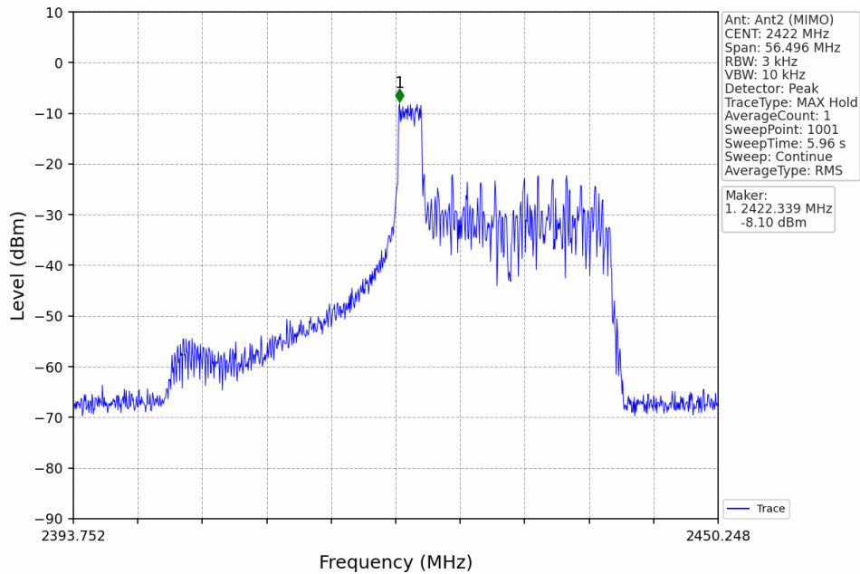
802.11ax(HEW40)_LCH_2422MHz_RU26_Mid_MIMO_NTNV
