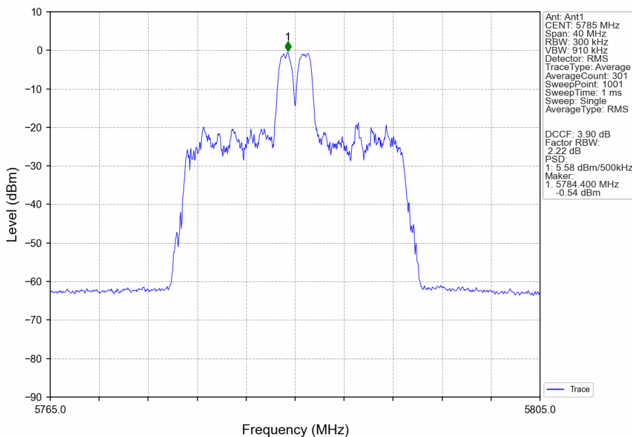
802.11ax(HEW20)_MCH_5785MHz_RU26_Mid_Ant1_NTNV
