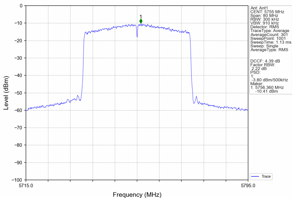
802.11ax(HEW40)_LCH_5755MHz_RU484_Left_MIMO_NTNV
