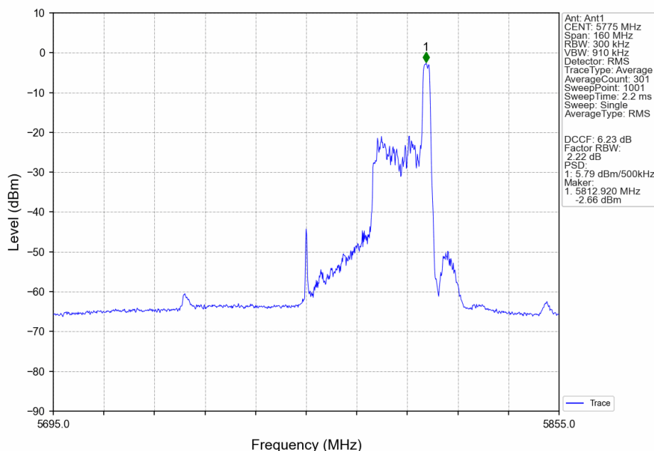
802.11ax(HEW80)_MCH_5775MHz_RU26_Right_MIMO_NTNV
