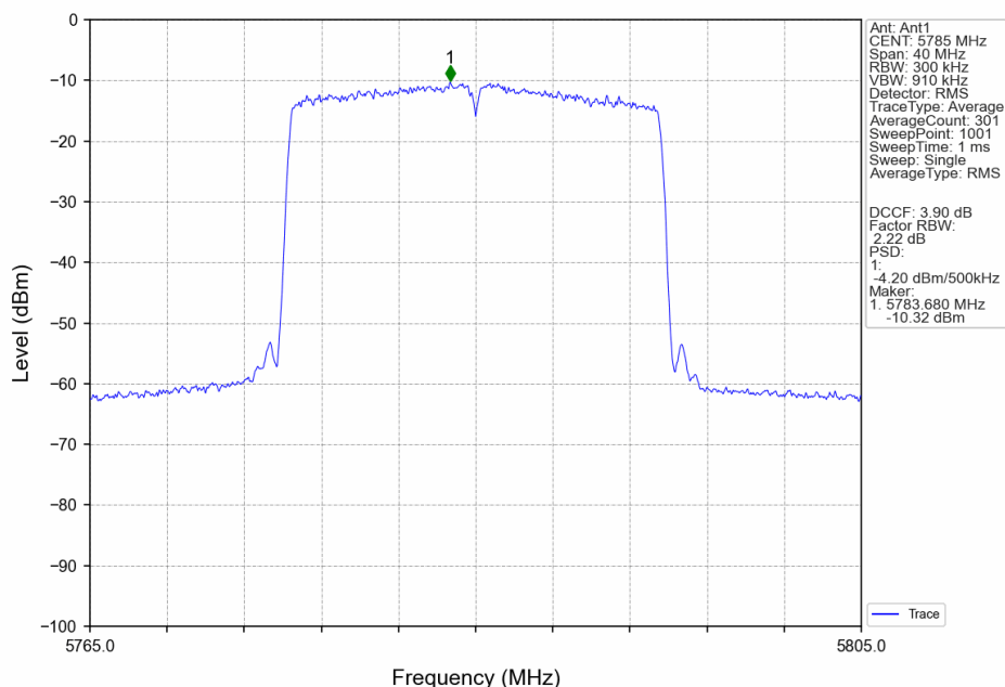
802.11ax(HEW20)_MCH_5785MHz_RU242_Left_MIMO_NTNV
