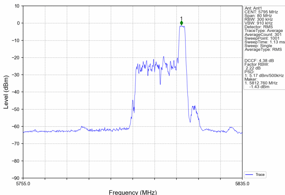
802.11ax(HEW40)_HCH_5795MHz_RU26_Right_Ant1_NTNV
