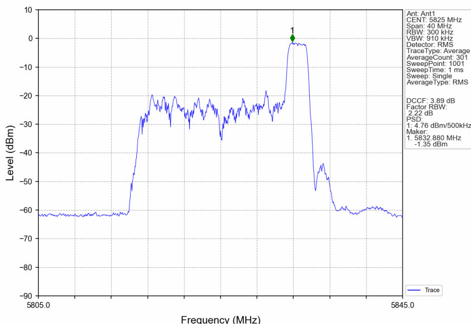
802.11ax(HEW20)_HCH_5825MHz_RU26_Right_Ant1_NTNV
