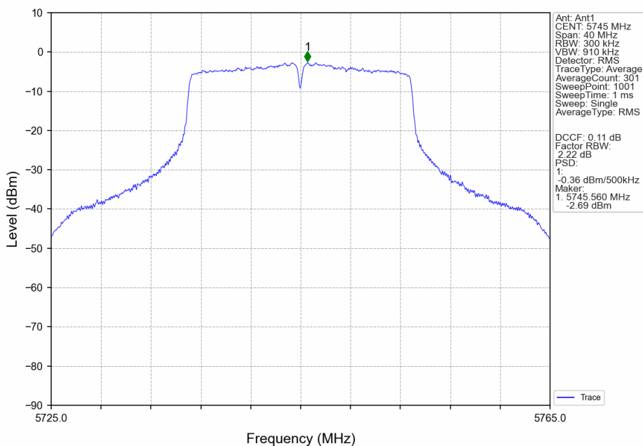
802.11n(HT20)_LCH_5745MHz_MIMO_NTNV
