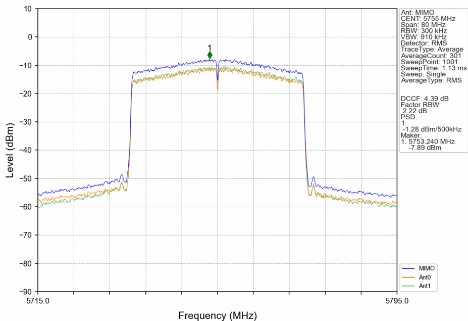
802.11ax(HEW40)_LCH_5755MHz_RU484_Left_MIMO_NTNV
