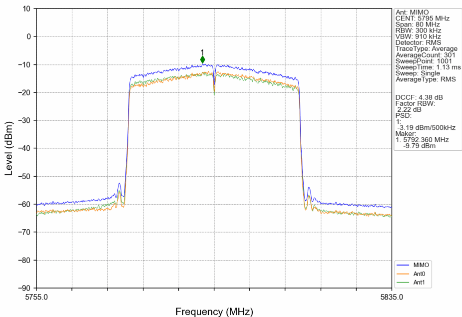
802.11ax(HEW40)_HCH_5795MHz_RU484_Left_MIMO_NTNV
