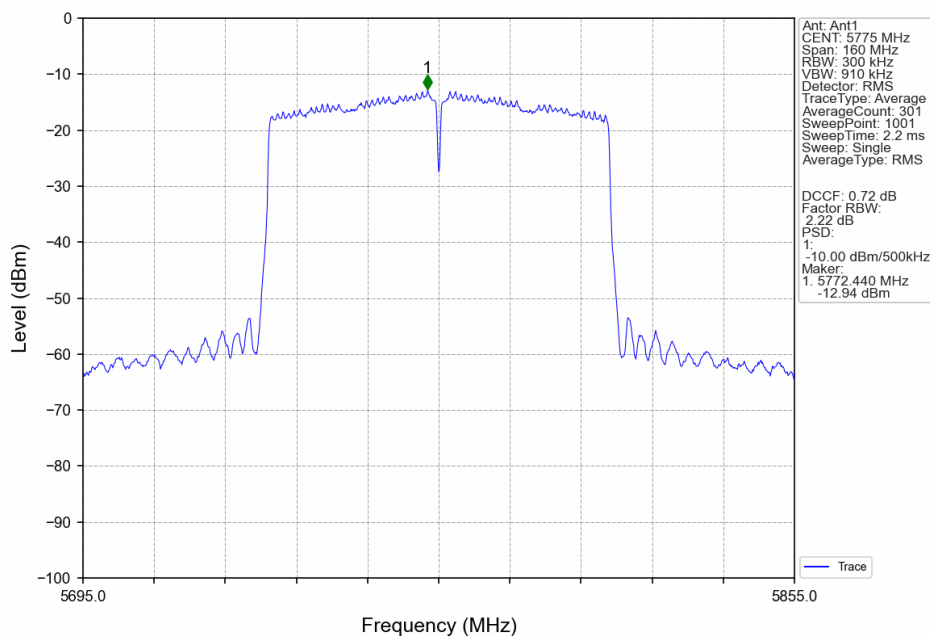
802.11ac(VHT80)_MCH_5775MHz_MIMO_NTNV
