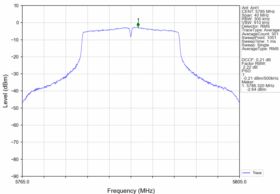
802.11ac(VHT20)_MCH_5785MHz_MIMO_NTNV
