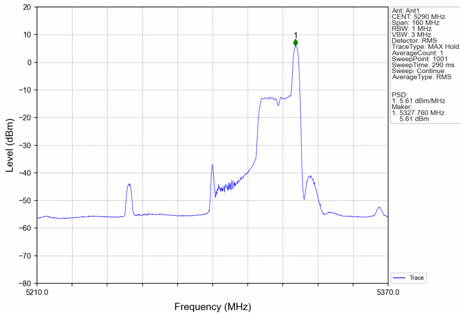
802.11ax(HEW80)_MCH_5290MHz_RU26_Right_MIMO_NTNV
