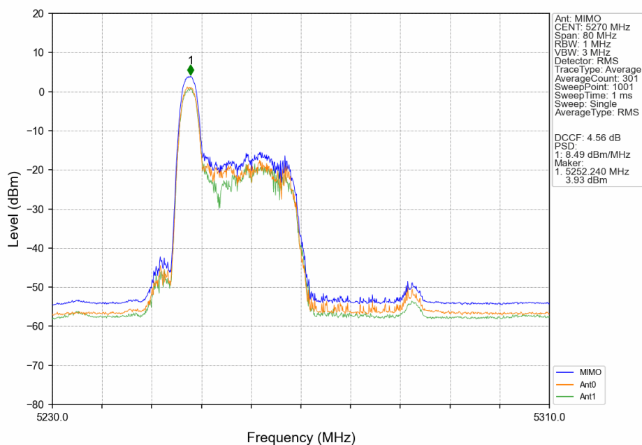
802.11ax(HEW40)_LCH_5270MHz_RU26_Left_MIMO_NTNV
