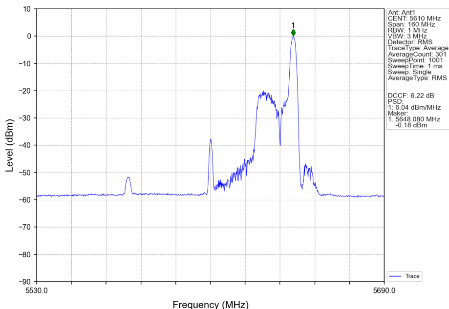
802.11ax(HEW80)_HCH_5610MHz_RU26_Right_MIMO_NTNV
