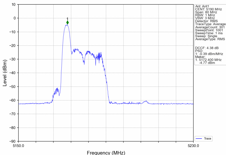
802.11ax(HEW40)_LCH_5190MHz_RU26_Left_MIMO_NTNV
