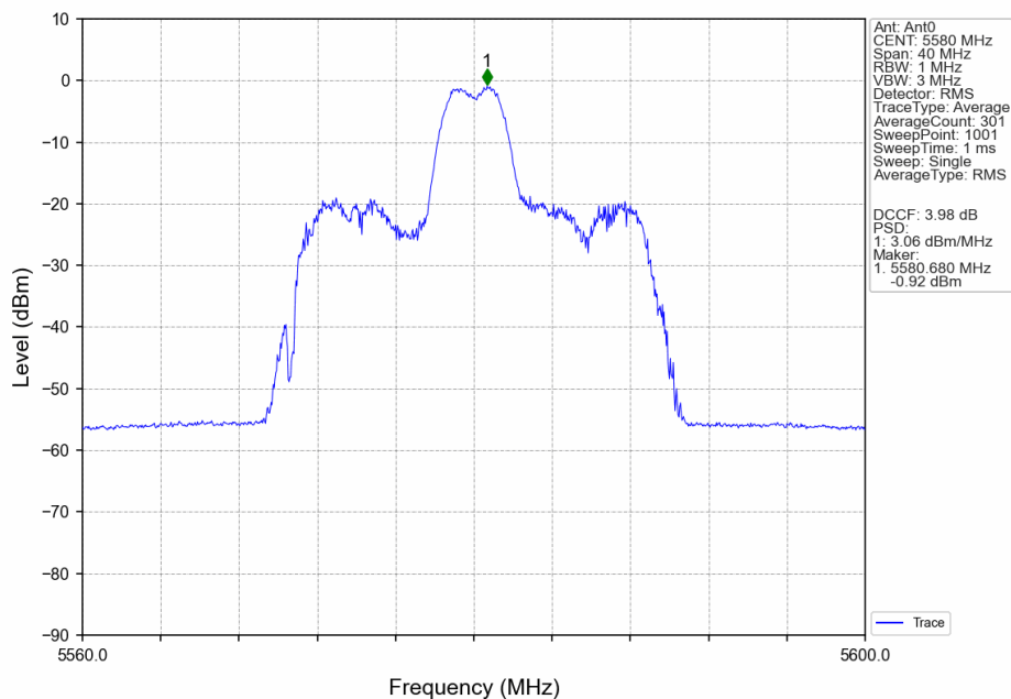
802.11ax(HEW20)_MCH_5580MHz_RU26_Mid_Ant0_NTNV
