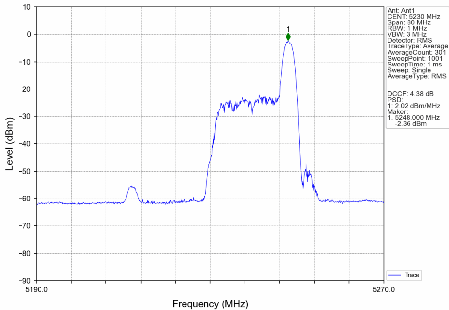
802.11ax(HEW40)_HCH_5230MHz_RU26_Right_MIMO_NTNV
