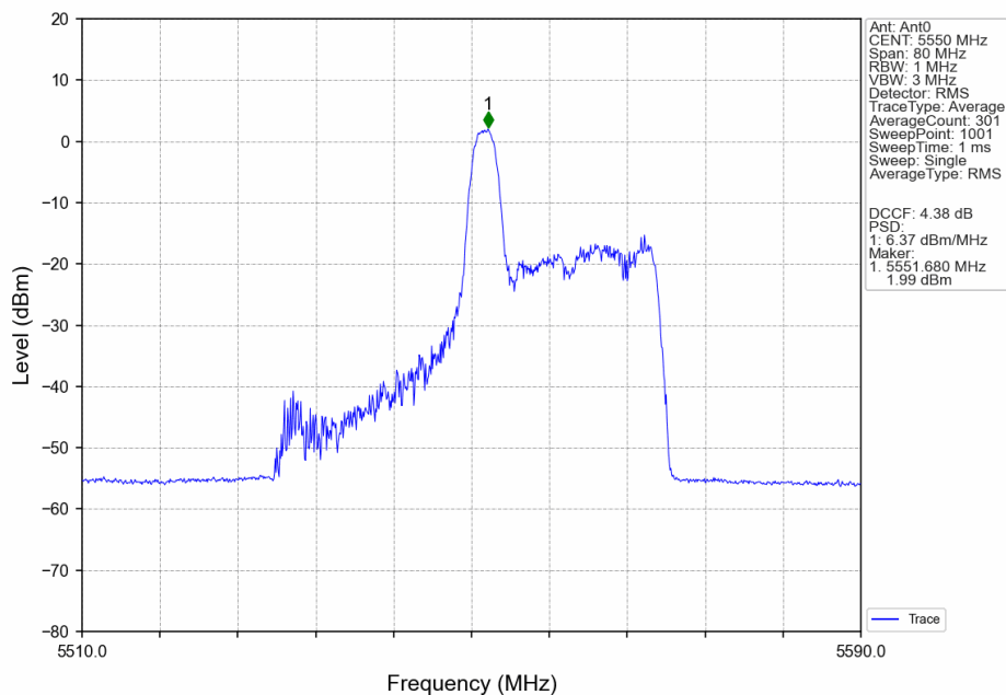
802.11ax(HEW40)_MCH_5550MHz_RU26_Mid_Ant0_NTNV
