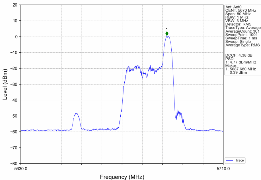
802.11ax(HEW40)_HCH_5670MHz_RU26_Right_Ant0_NTNV
