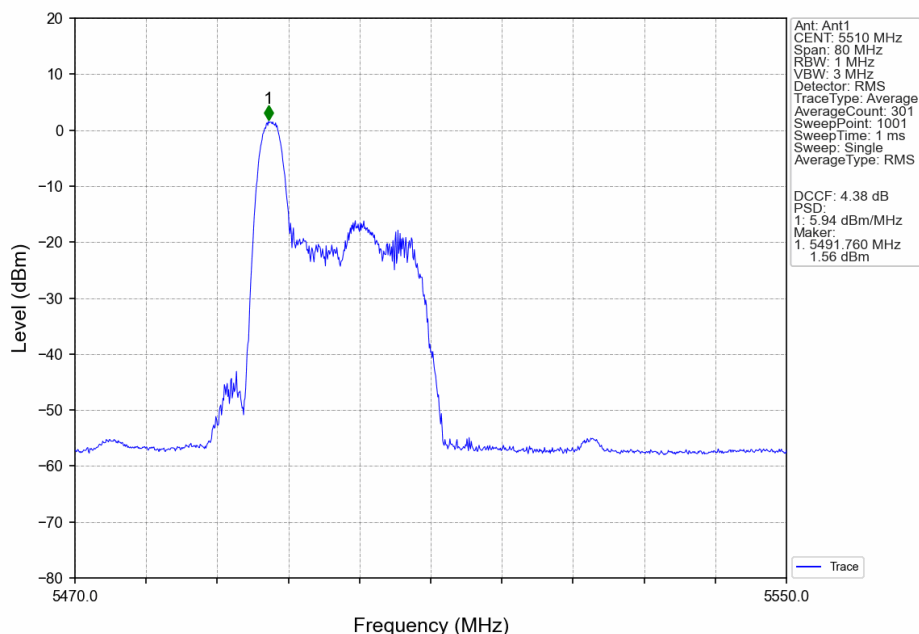
802.11ax(HEW40)_LCH_5510MHz_RU26_Left_MIMO_NTNV
