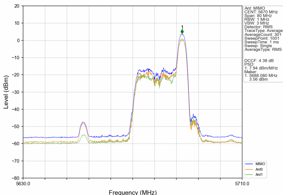
802.11ax(HEW40)_HCH_5670MHz_RU26_Right_MIMO_NTNV
