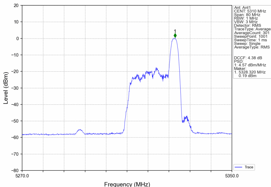
802.11ax(HEW40)_HCH_5310MHz_RU26_Right_MIMO_NTNV
