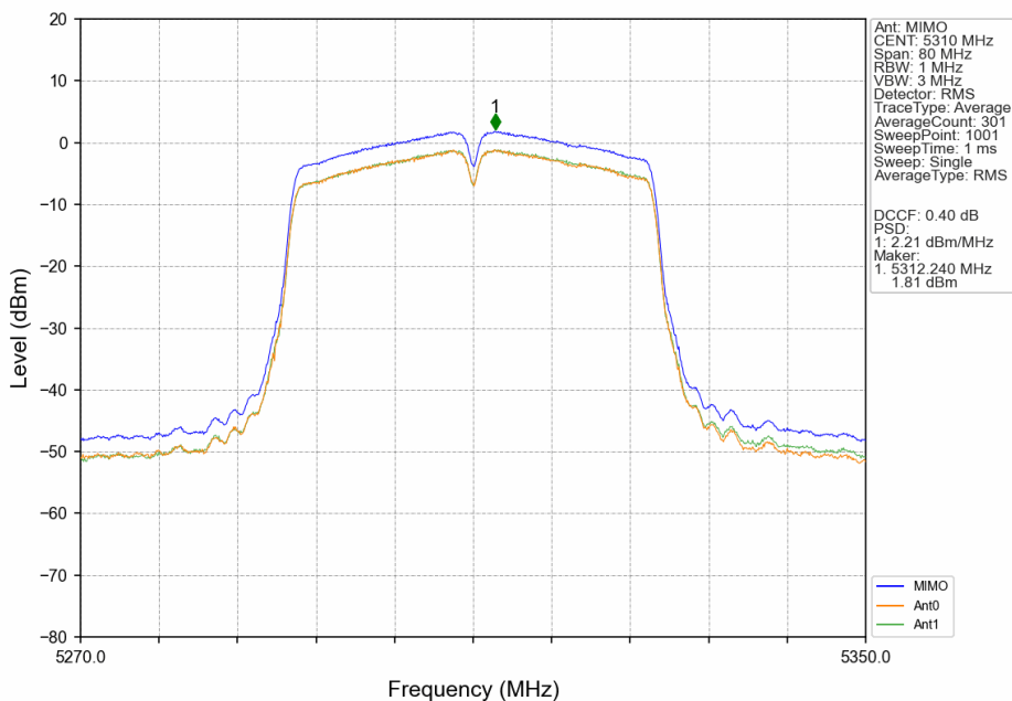
802.11ac(VHT40)_HCH_5310MHz_MIMO_NTNV
