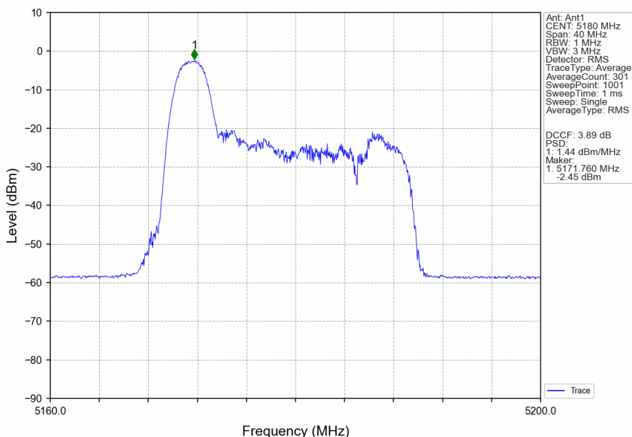
802.11ax(HEW20)_LCH_5180MHz_RU26_Left_MIMO_NTNV
