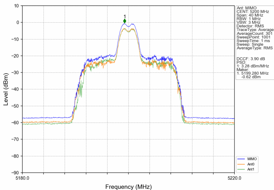
802.11ax(HEW20)_MCH_5200MHz_RU26_Mid_MIMO_NTNV
