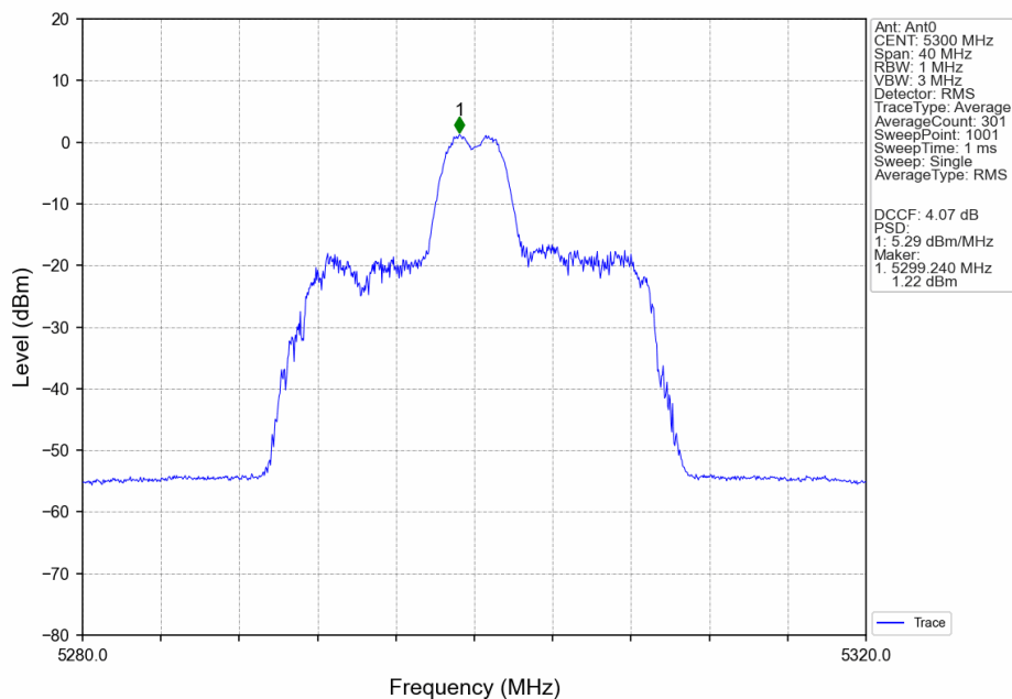
802.11ax(HEW20)_MCH_5300MHz_RU26_Mid_Ant0_NTNV
