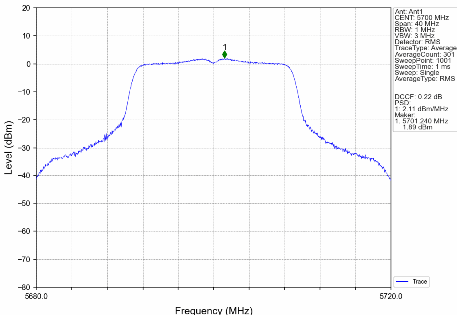
802.11ac(VHT20)_HCH_5700MHz_MIMO_NTNV
