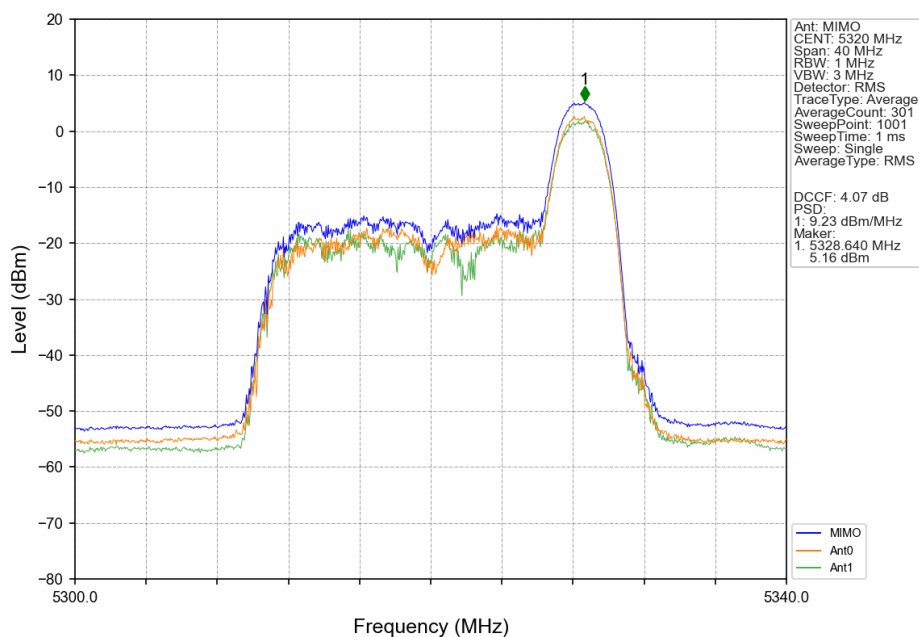
802.11ax(HEW20)_HCH_5320MHz_RU26_Right_MIMO_NTNV
