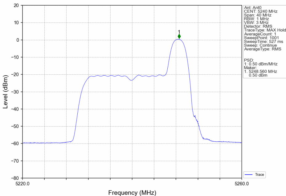
802.11ax(HEW20)_HCH_5240MHz_RU26_Right_Ant0_NTNV
