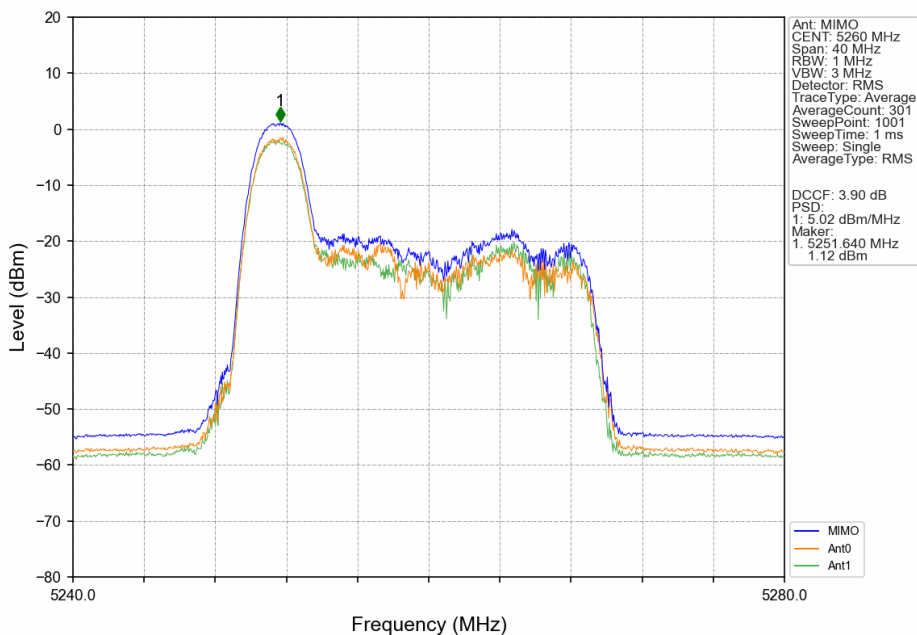
802.11ax(HEW20)_LCH_5260MHz_RU26_Left_MIMO_NTNV
