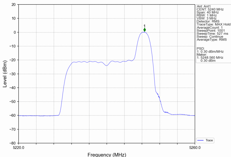
802.11ax(HEW20)_HCH_5240MHz_RU26_Right_MIMO_NTNV
