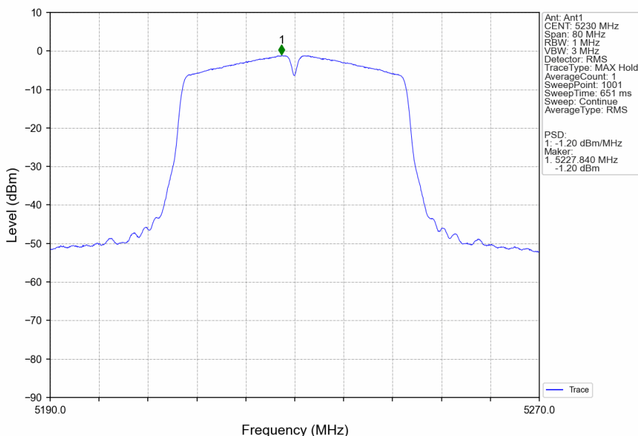
802.11n(HT40)_HCH_5230MHz_MIMO_NTNV
