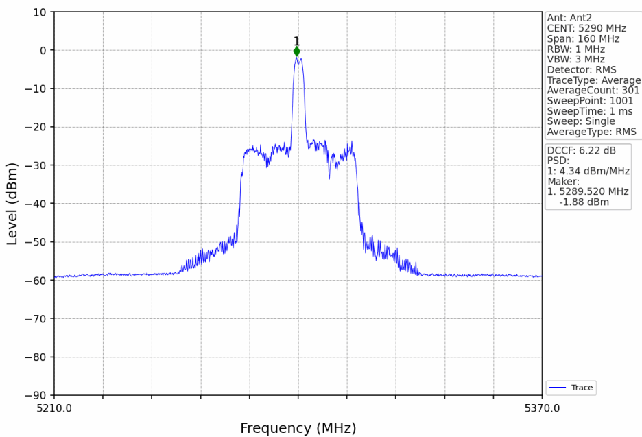
802.11ax(HEW80)_MCH_5290MHz_RU26_Mid_Ant2_NTNV
