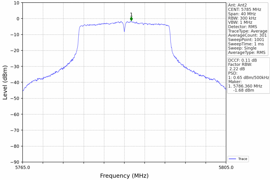
802.11ac(VHT20)_MCH_5785MHz_MIMO_NTNV
