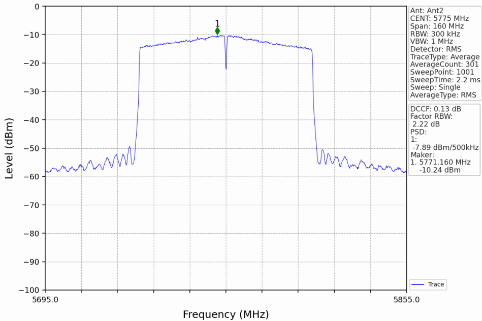
802.11ac(VHT80)_MCH_5775MHz_MIMO_NTNV
