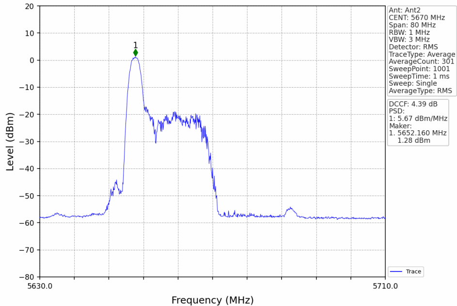
802.11ax(HEW40)_HCH_5670MHz_RU26_Left_MIMO_NTNV
