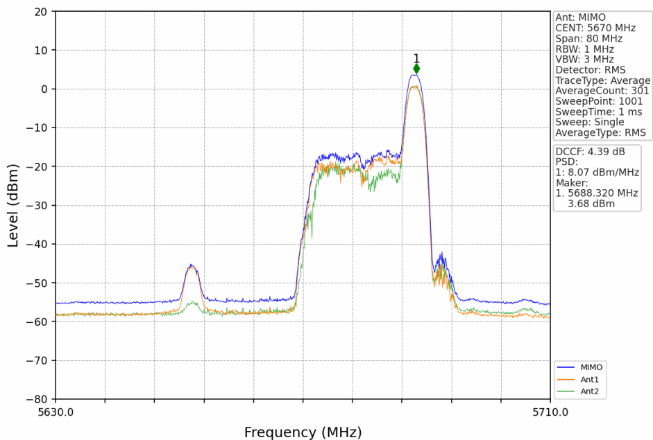
802.11ax(HEW40)_HCH_5670MHz_RU26_Right_MIMO_NTNV
