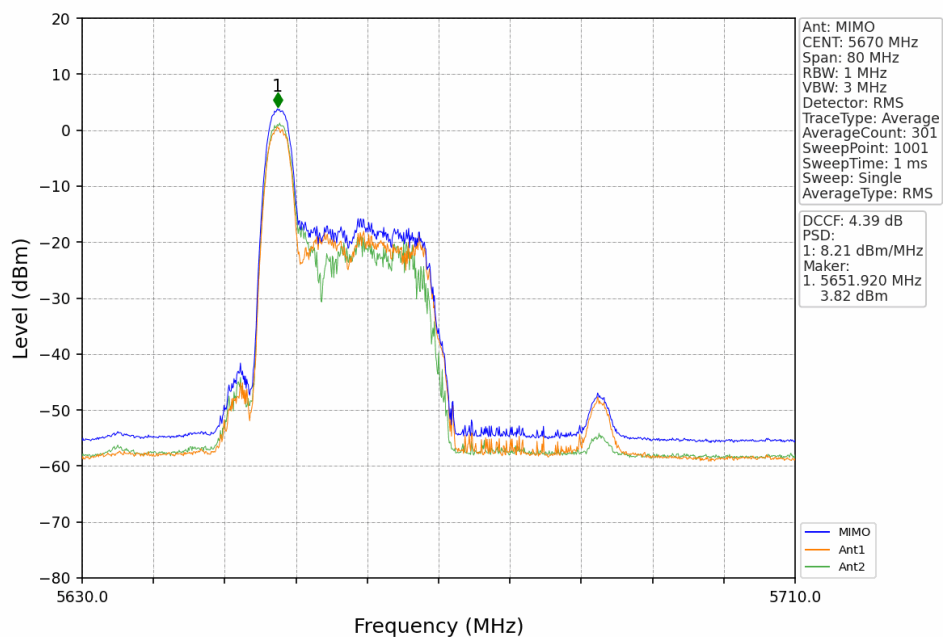
802.11ax(HEW40)_HCH_5670MHz_RU26_Left_MIMO_NTNV
