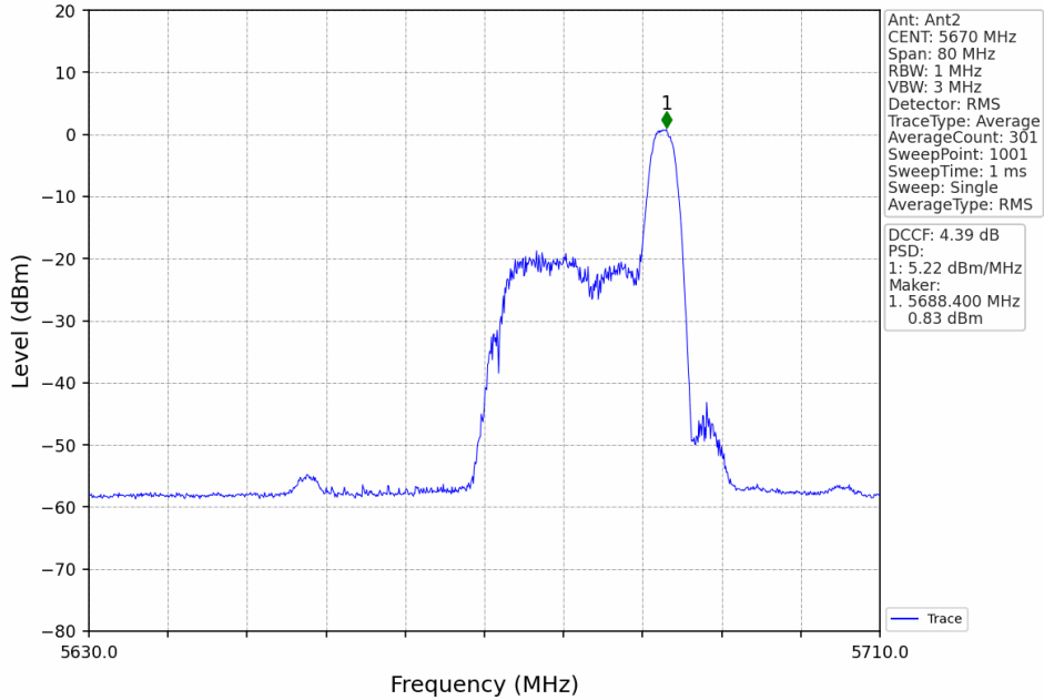
802.11ax(HEW40)_HCH_5670MHz_RU26_Right_MIMO_NTNV
