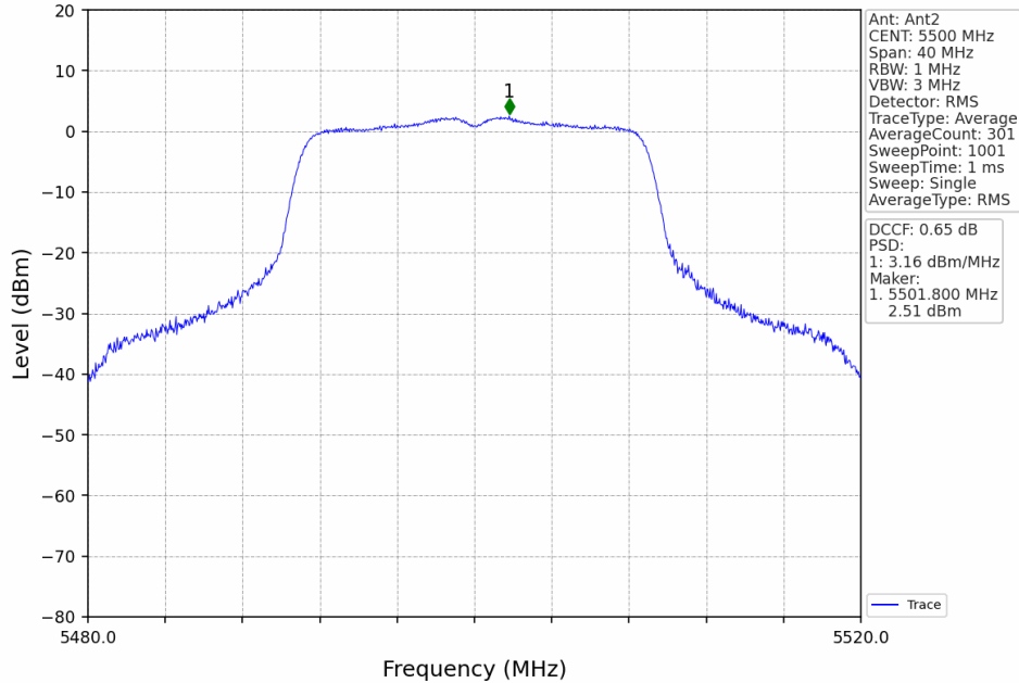
802.11ac(VHT20)_LCH_5500MHz_MIMO_NTNV
