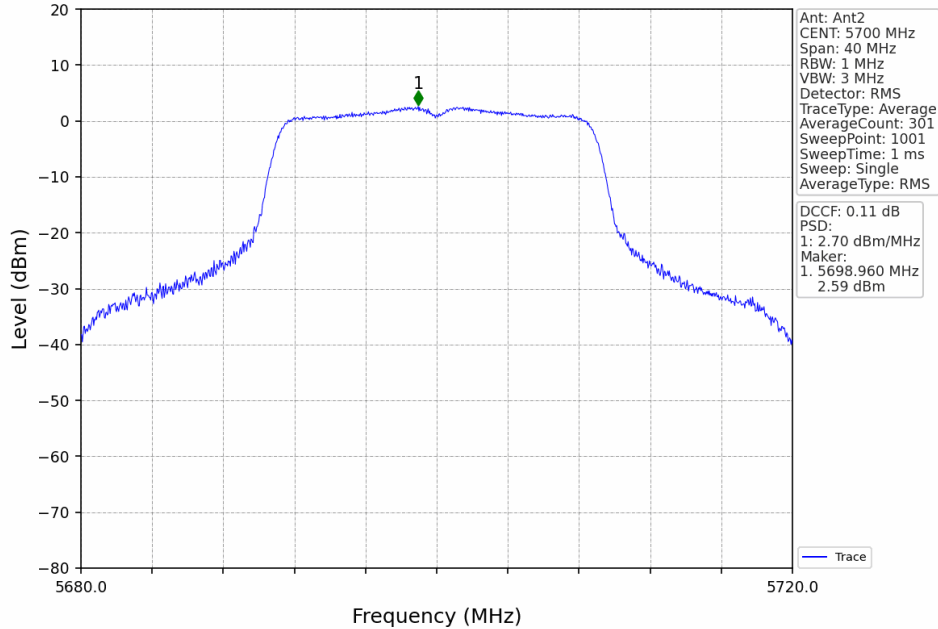
802.11ac(VHT20)_HCH_5700MHz_MIMO_NTNV
