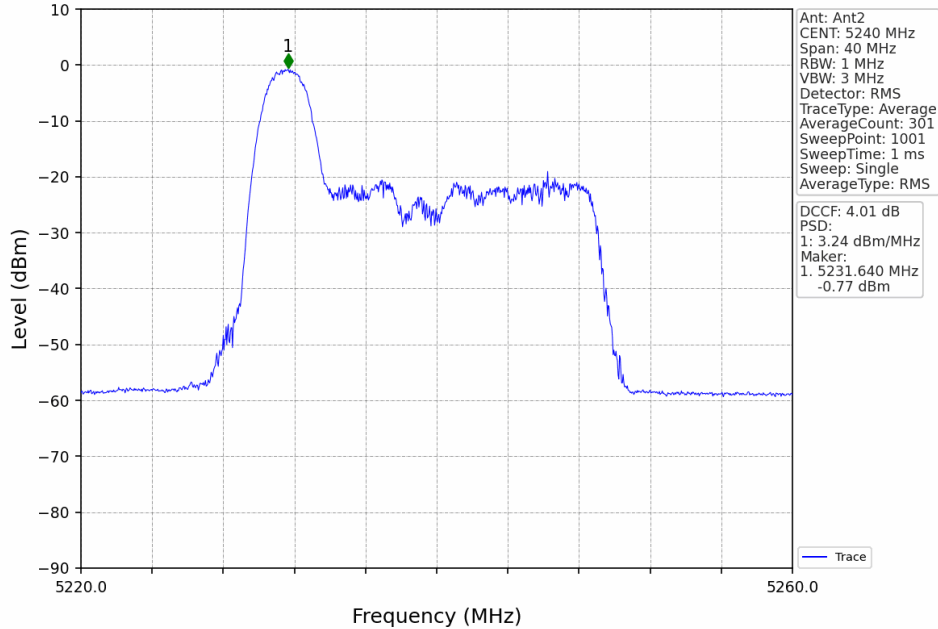
802.11ax(HEW20)_HCH_5240MHz_RU26_Left_MIMO_NTNV
