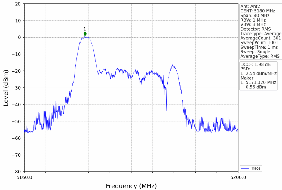
802.11ax(HEW20)_LCH_5180MHz_RU26_Left_MIMO_NTNV
