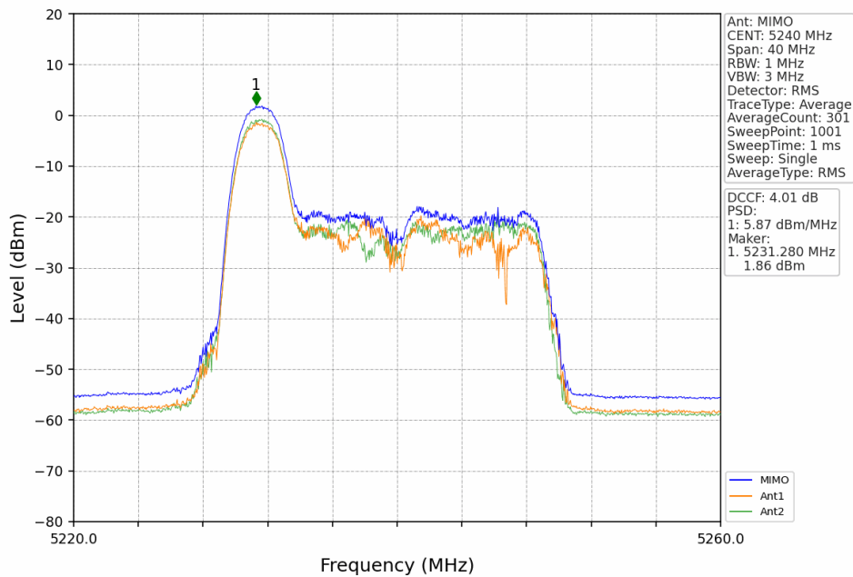
802.11ax(HEW20)_HCH_5240MHz_RU26_Left_MIMO_NTNV
