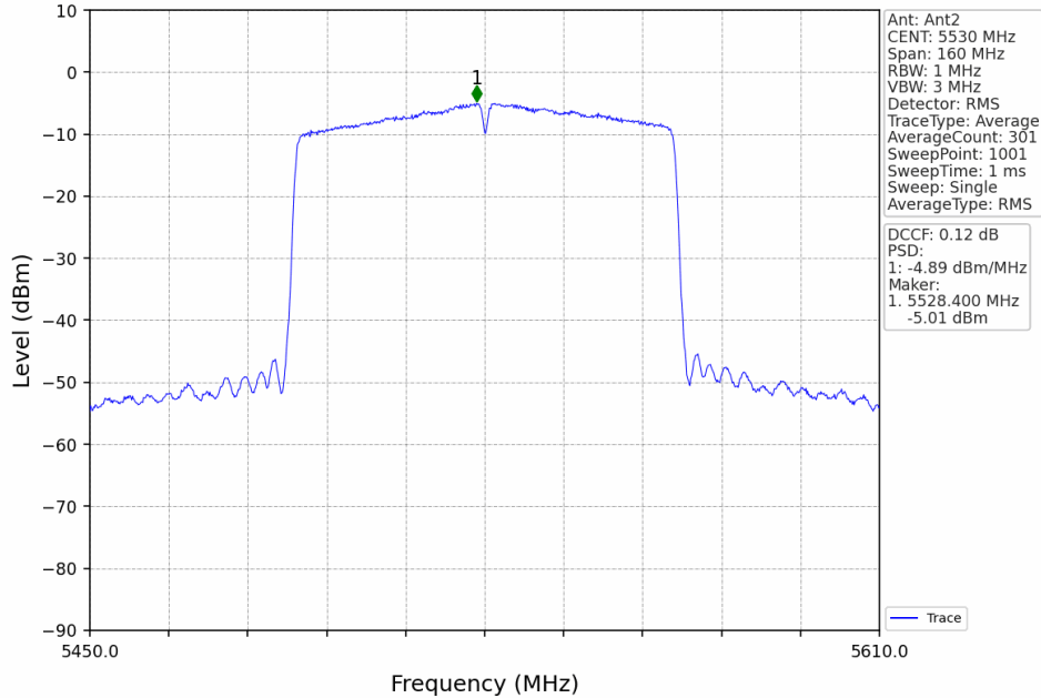
802.11ac(VHT80)_LCH_5530MHz_MIMO_NTNV
