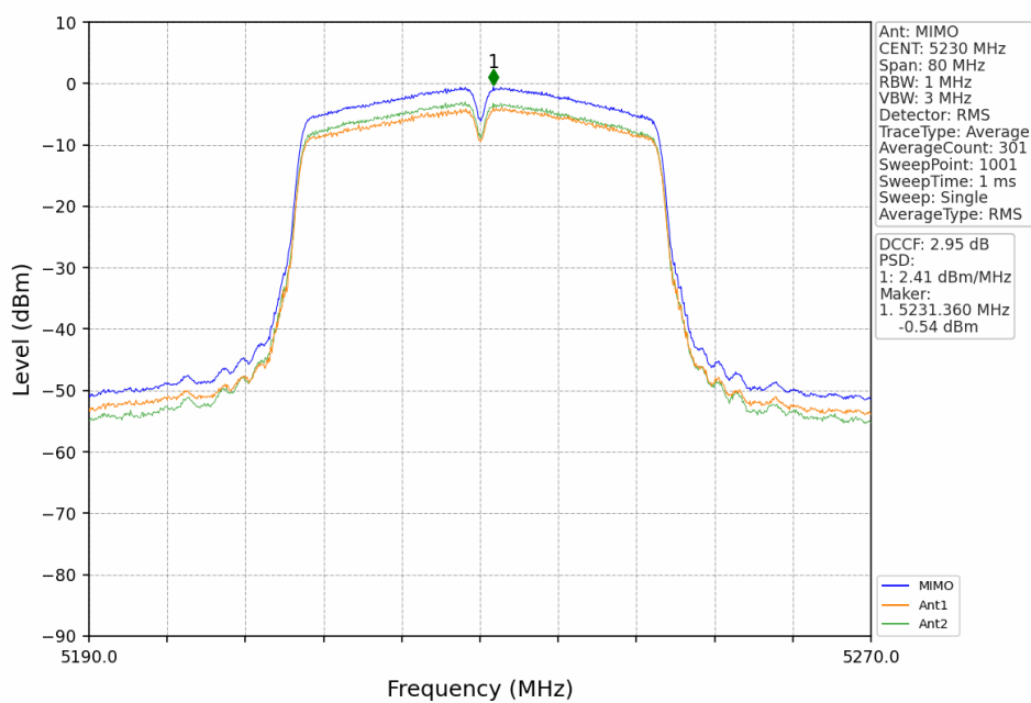
802.11ac(VHT40)_HCH_5230MHz_MIMO_NTNV
