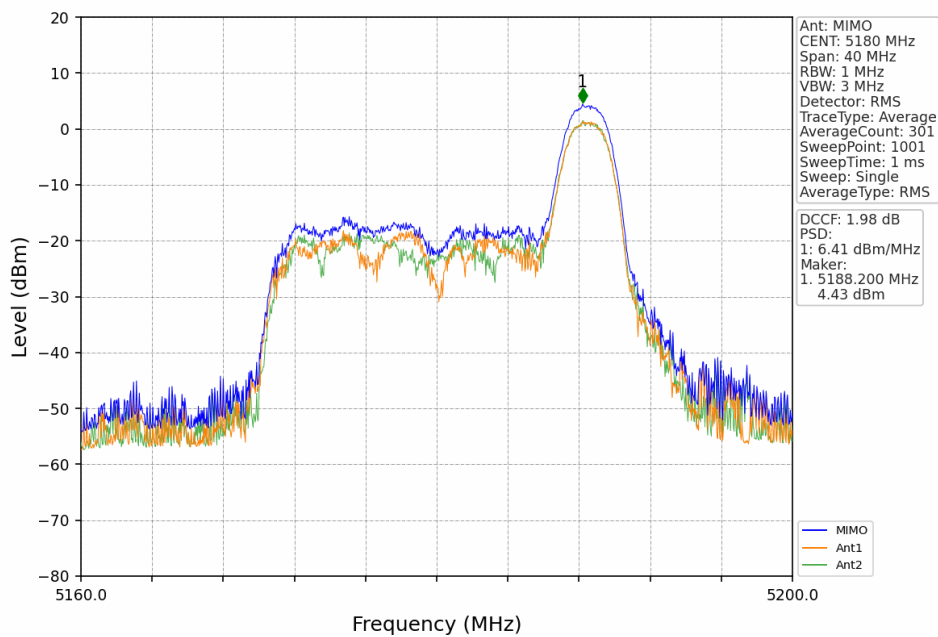
802.11ax(HEW20)_LCH_5180MHz_RU26_Right_MIMO_NTNV
