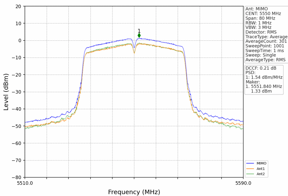
802.11ac(VHT40)_MCH_5550MHz_MIMO_NTNV
