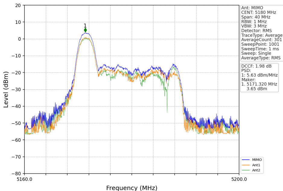
802.11ax(HEW20)_LCH_5180MHz_RU26_Left_MIMO_NTNV
