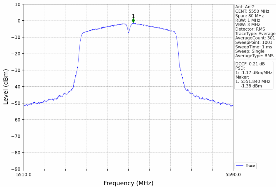
802.11ac(VHT40)_MCH_5550MHz_MIMO_NTNV
