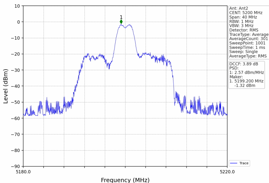
802.11ax(HEW20)_MCH_5200MHz_RU26_Mid_Ant2_NTNV
