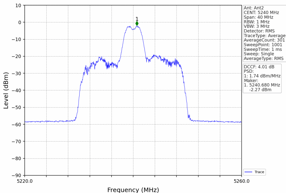
802.11ax(HEW20)_HCH_5240MHz_RU26_Mid_Ant2_NTNV
