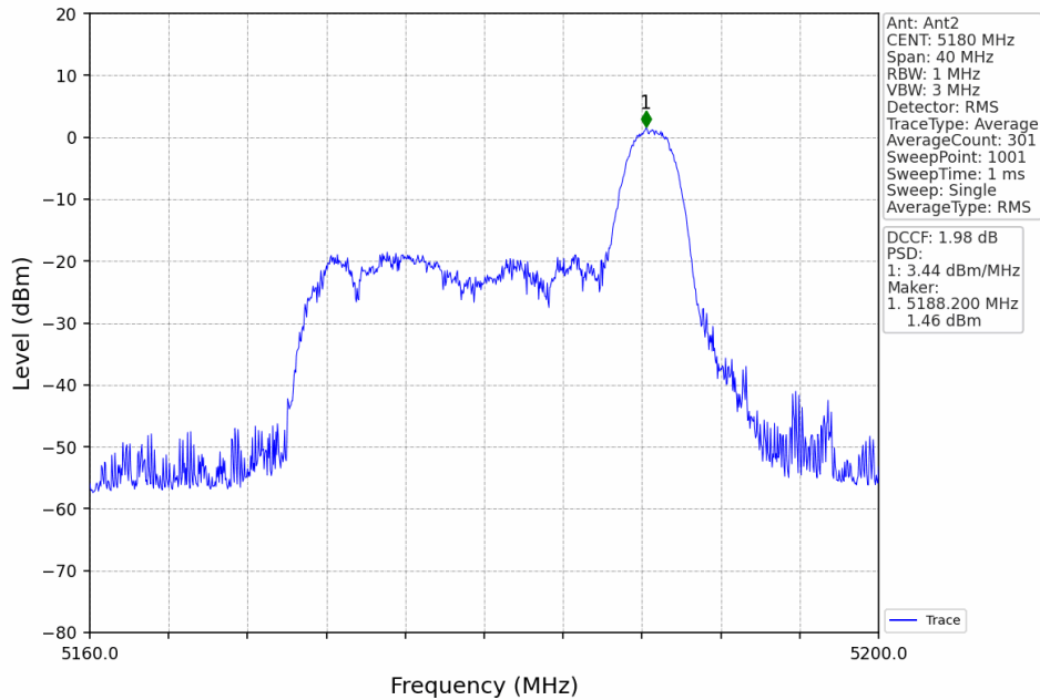
802.11ax(HEW20)_LCH_5180MHz_RU26_Right_MIMO_NTNV
