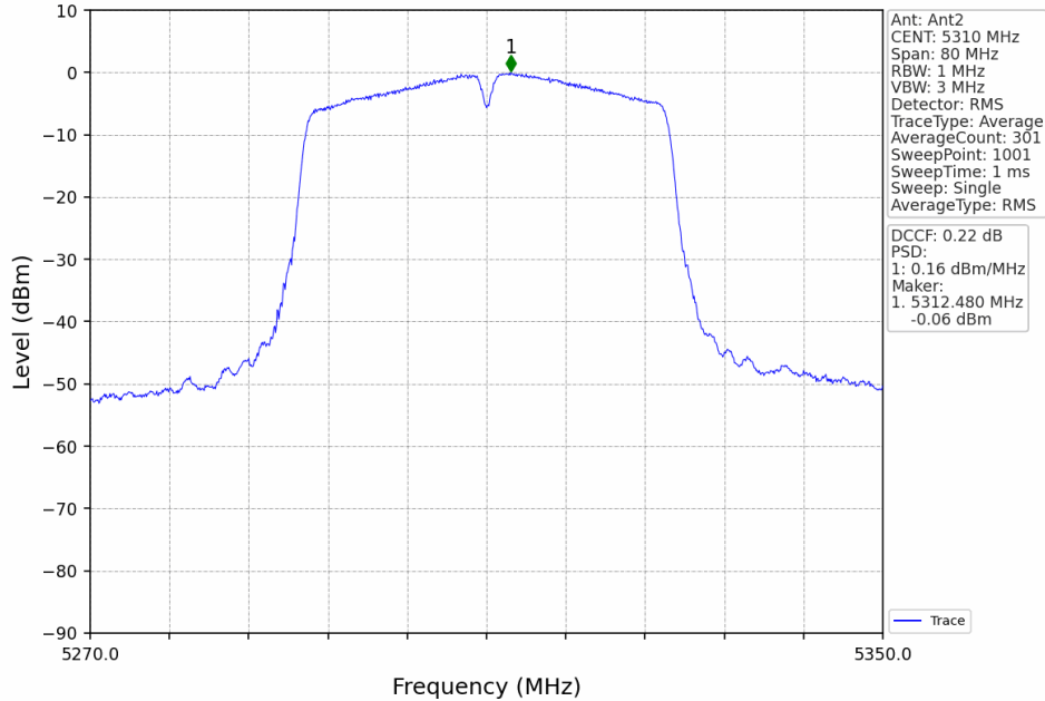
802.11ac(VHT40)_HCH_5310MHz_MIMO_NTNV
