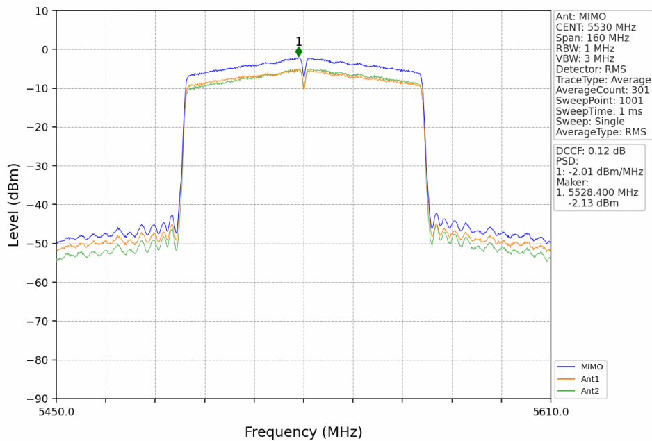
802.11ac(VHT80)_LCH_5530MHz_MIMO_NTNV
