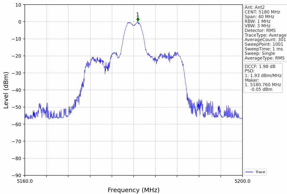
802.11ax(HEW20)_LCH_5180MHz_RU26_Mid_Ant2_NTNV
