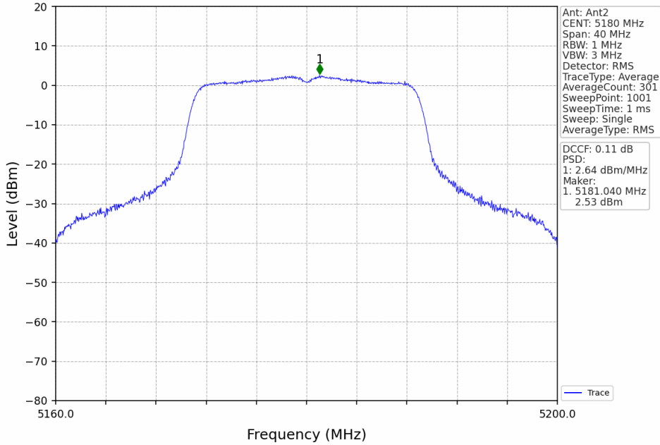
802.11ac(VHT20)_LCH_5180MHz_MIMO_NTNV
