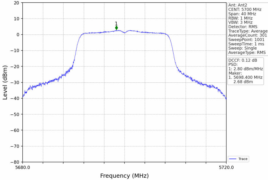
802.11n(HT20)_HCH_5700MHz_MIMO_NTNV
