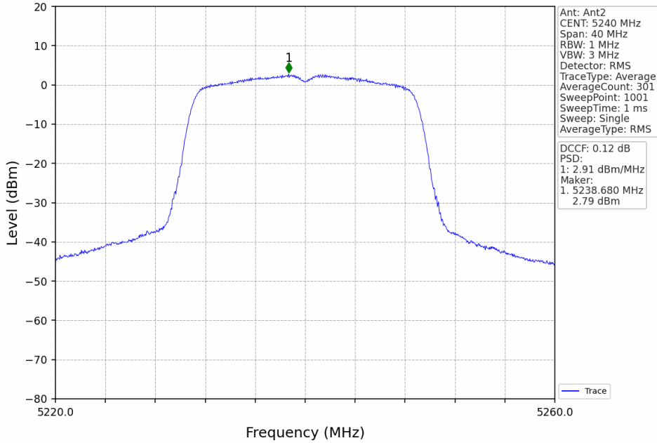
802.11ac(VHT20)_HCH_5240MHz_MIMO_NTNV
