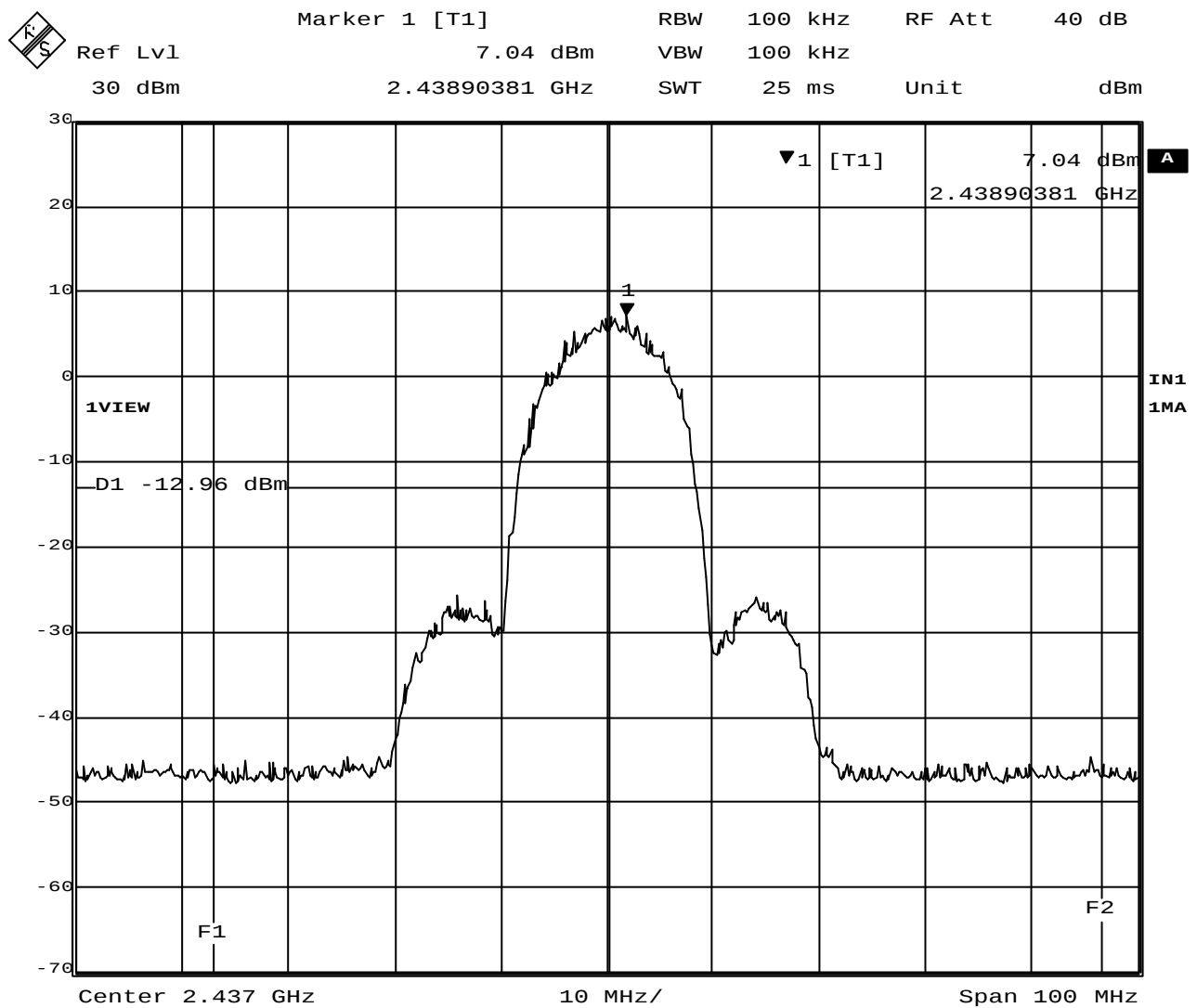
Plot 2-5. Out of band emissions around 2437MHz
