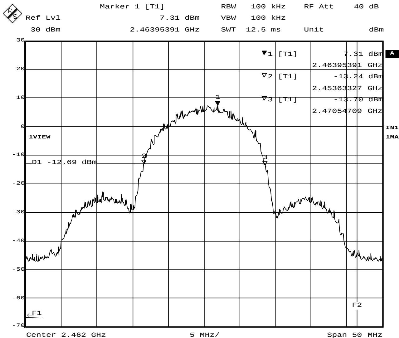
Plot 2-3. 20dB BW at 2462MHz
