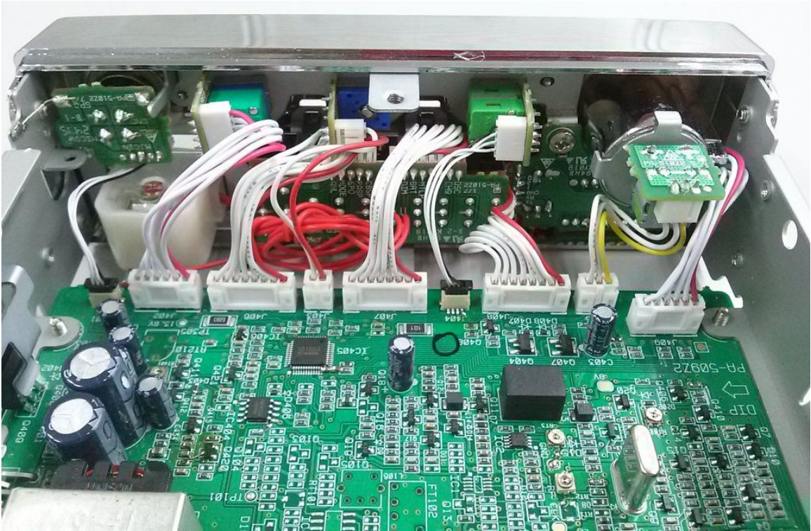
PC68LTD Front Inner View
