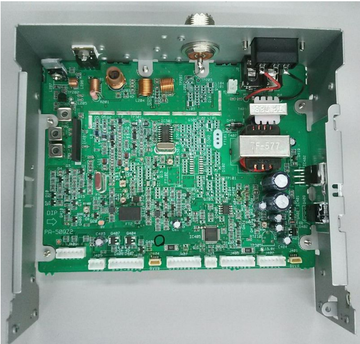
PC68LTD Main Top View
