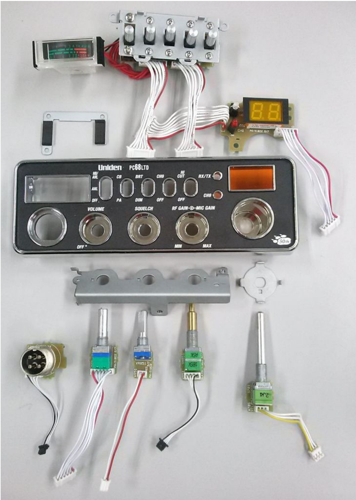
PC68LTD Front Top
