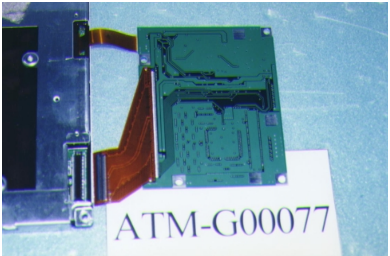
Figure 13 Video Board (Foil Side)
