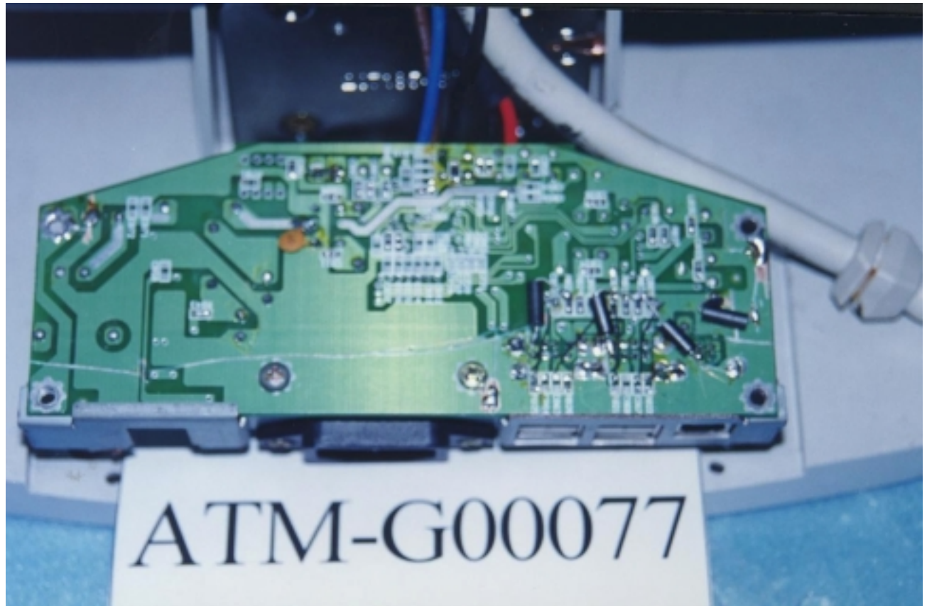
Figure 21 PC Board of USB HUB
