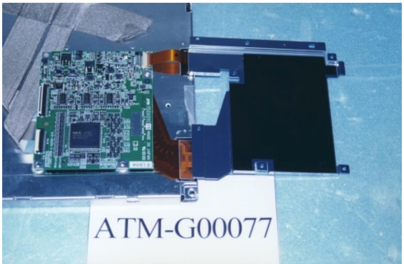
Figure 12 Video Board (Component Side)
