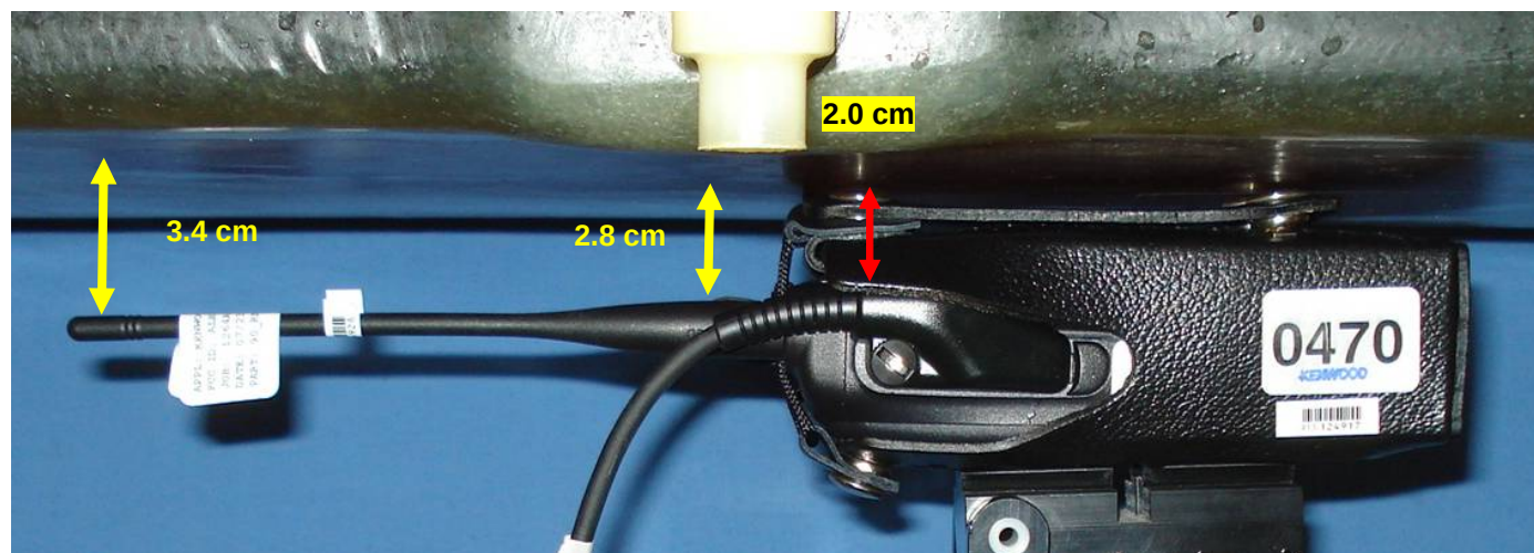
Body-worn SAR Configuration - Antenna 1, Audio G1a
