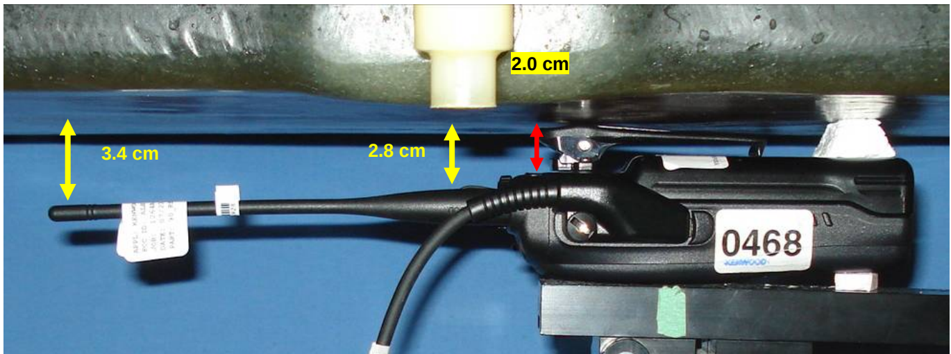
Body-worn SAR Configuration - Antenna 1, Battery b, Audio G1a
