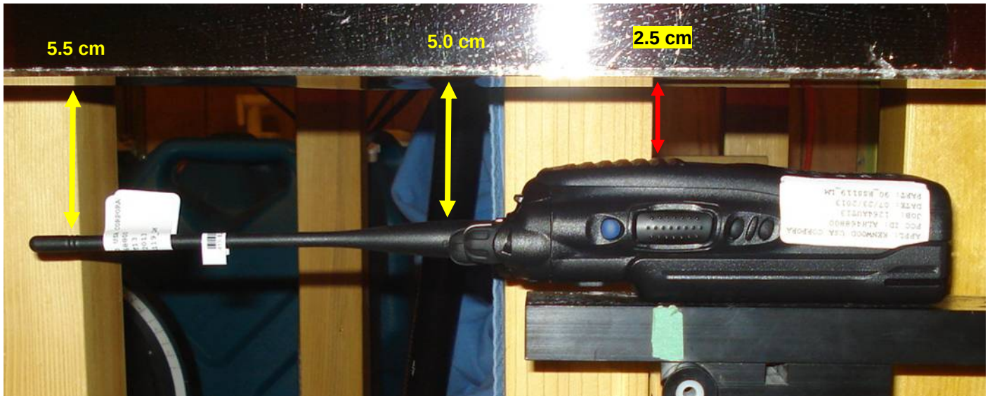
Face-held SAR Configuration - Antenna 1, Battery a
