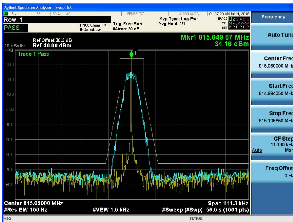
815.05 MHz_High
