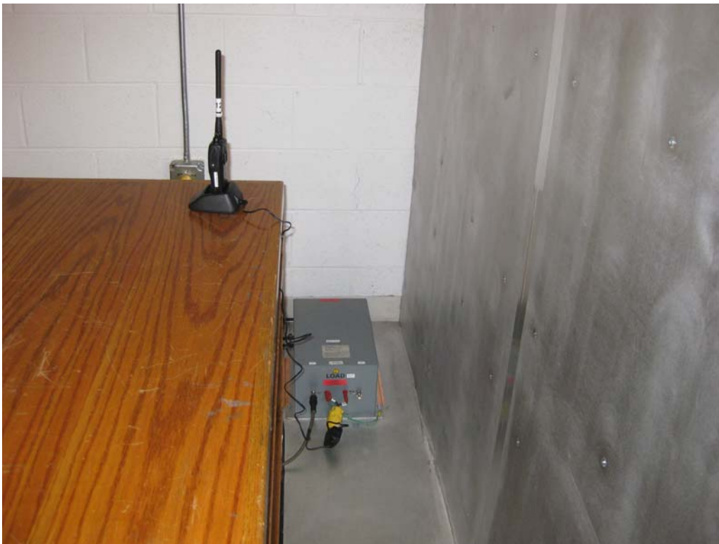
Conducted Emissions #2
