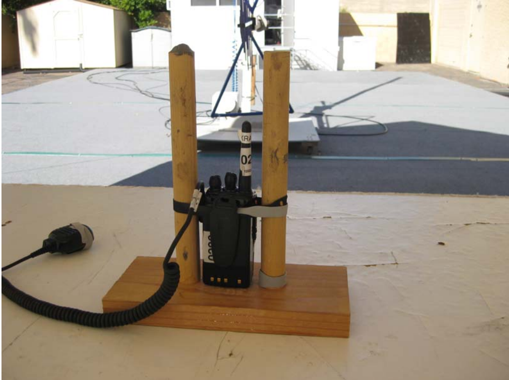
Radiated Spur Emission below 1 GHz #1
