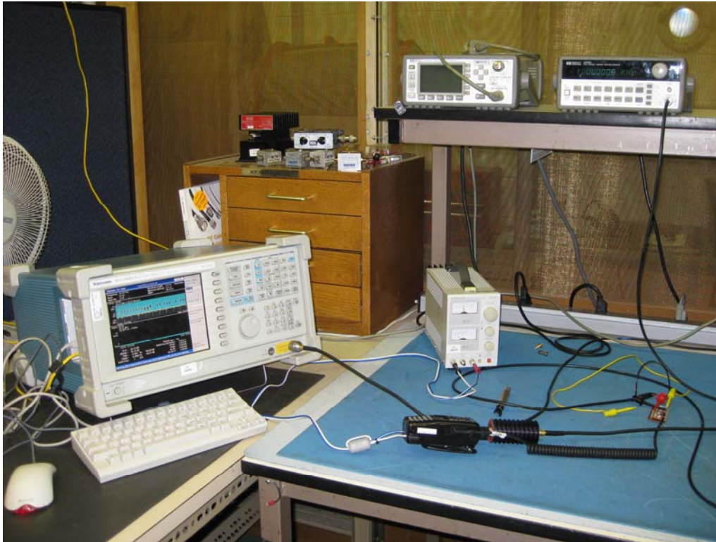
Radiated Spur Emission above 1 GHz #1
