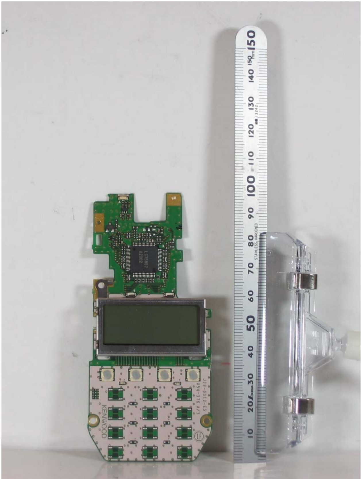
NX-320-K2 Display Unit
