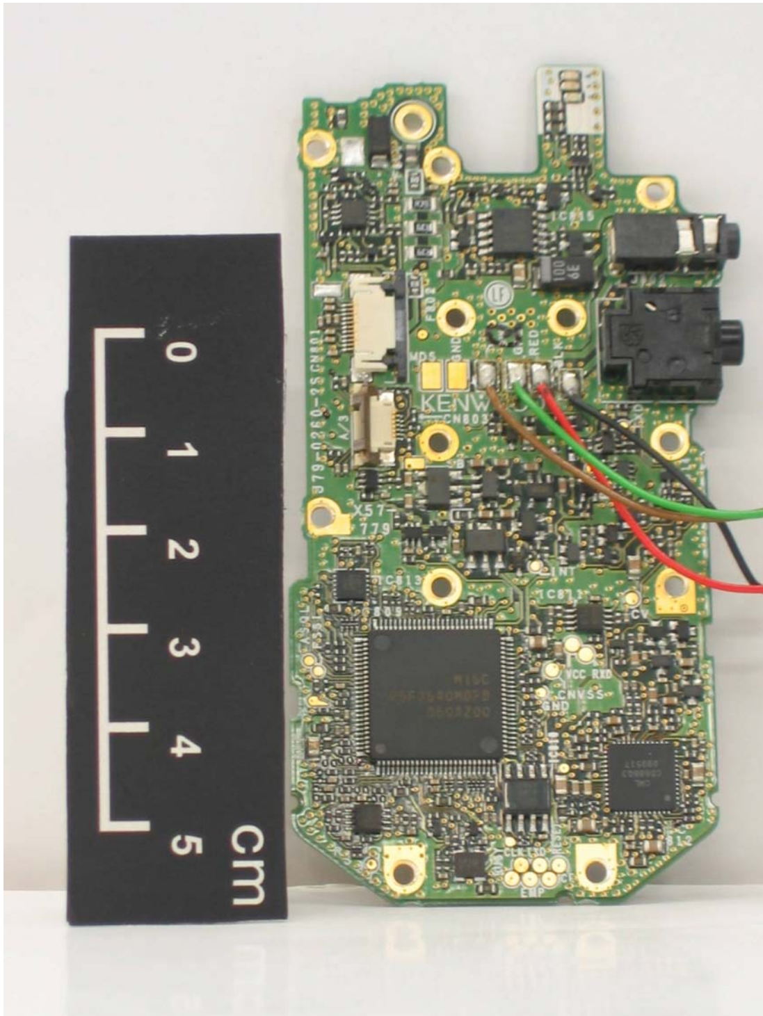
Component Side View
