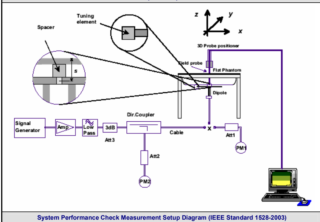
835 MHz SPEAG Validation Dipole Setup with Barski Planar Phantom
