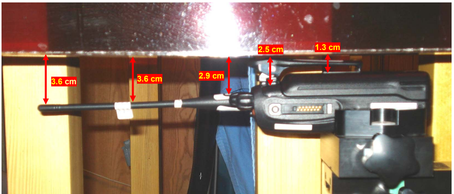
ANTENNA A - Body-worn Test Setup with KRA-32 Whip Antenna & Ni-MH Batt "b" – 2.5 cm Belt-Clip Spacing - Battery Housing Parallel to Phantom
