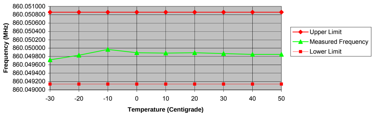
860.05 MHz Frequency Stability vs. Temperature
