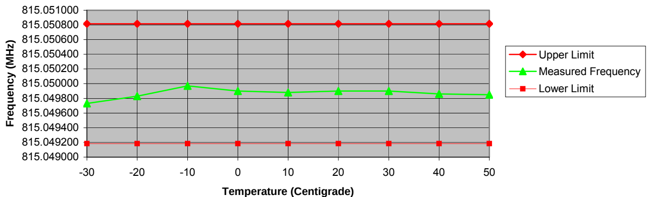
815.05 MHz Frequency Stability vs. Temperature
