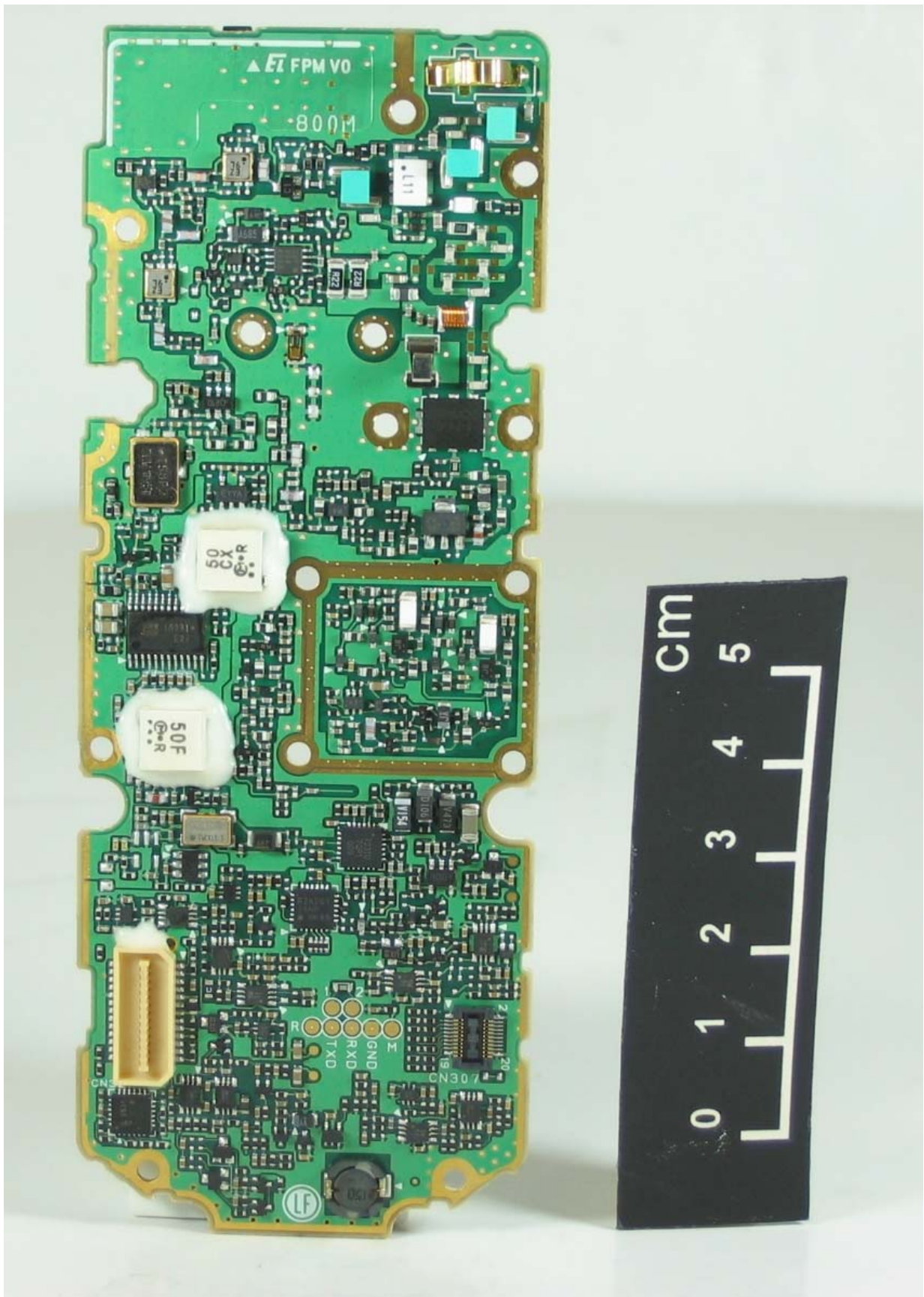
TXRX UNIT
