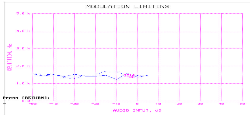
N Graph
