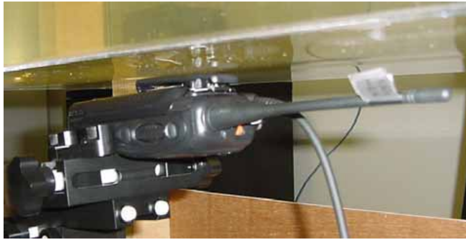
Body SAR with KRA-27M antenna, KBH-10 Belt Clip and Thick Battery
