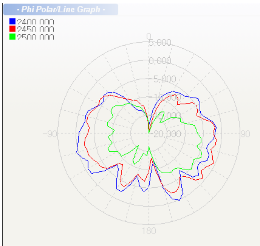
(c) Elevation2 Plane (XZ) – Vertical Polarization
