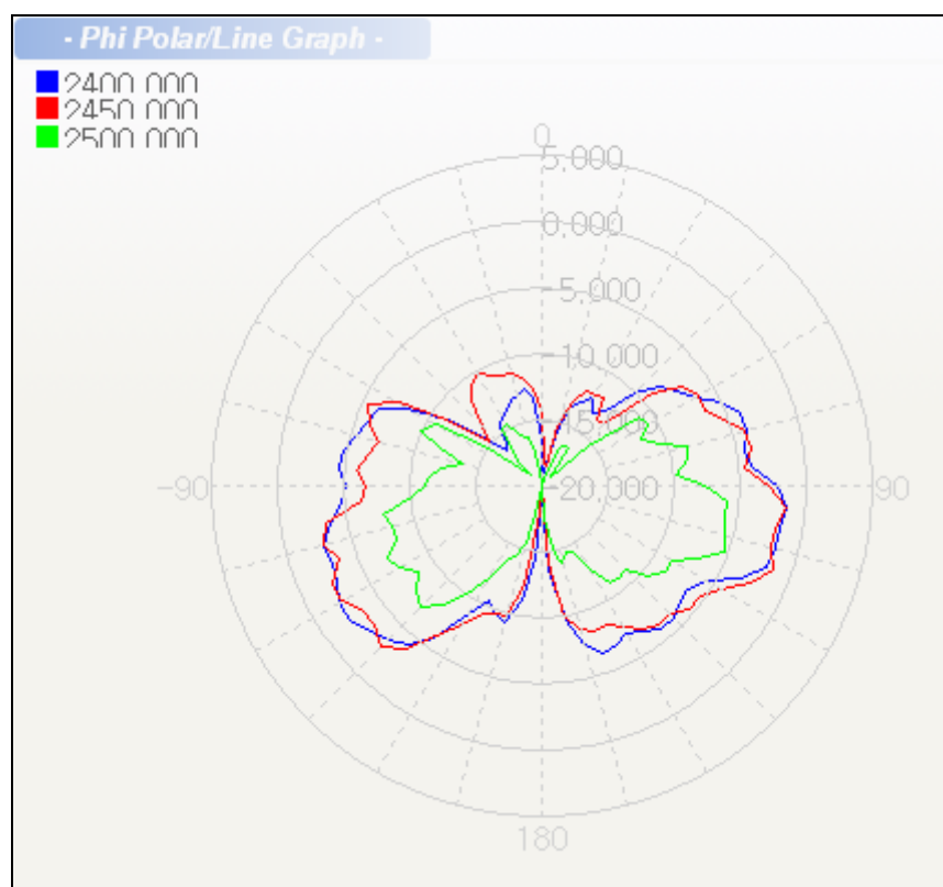
(c) Elevation2 Plane (XZ) – Vertical Polarization
