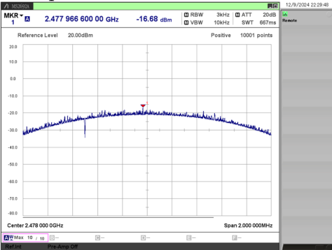
[ 2 Mbps / 2478 MHz ]
